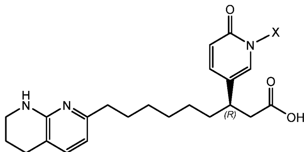
(Structure 31b),
