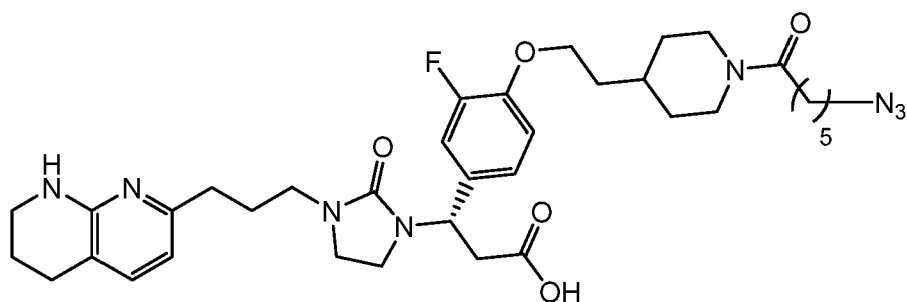
(Structure 2.2c).
