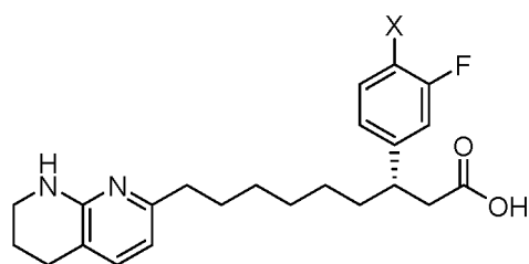
(Structure 31b),
