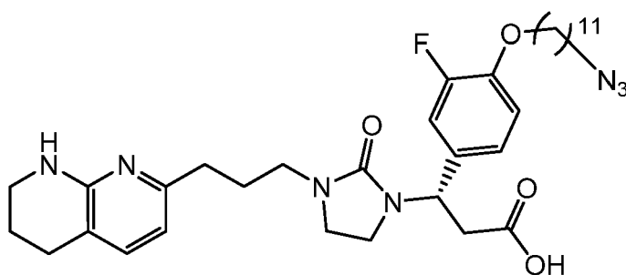
(Structure 2.1c).
