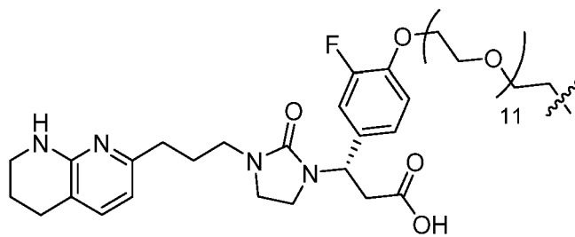
(Structure 2.8a);
