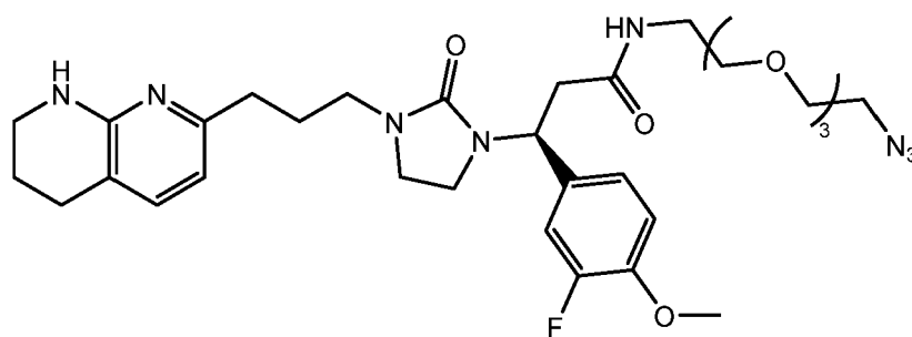
(Structure 2.7c).
