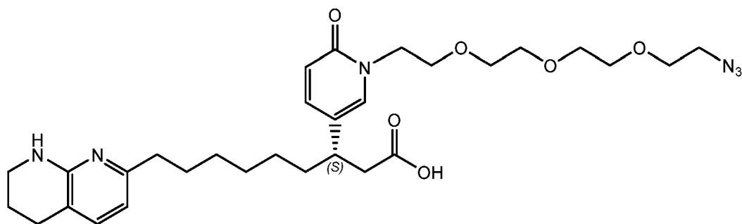
(Structure 30c).
