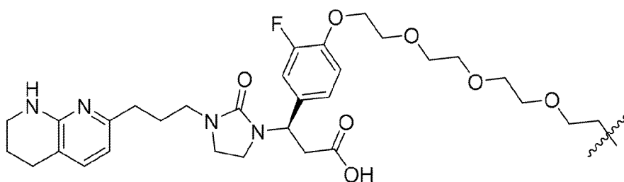
(Structure 2.11a);
