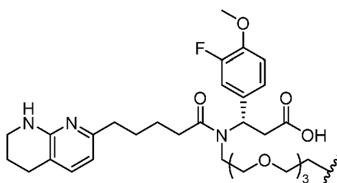
(Structure 33a);
