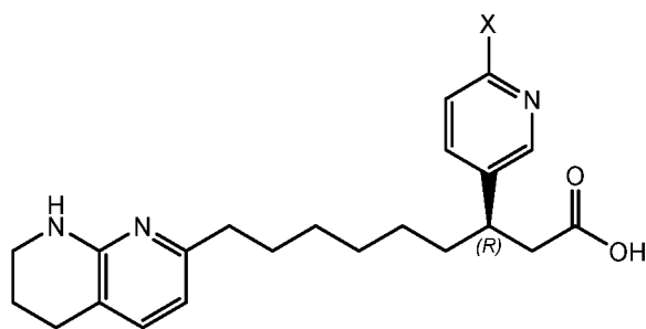
(Structure 28b),
