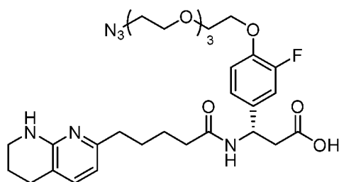
(Structure 37c).
