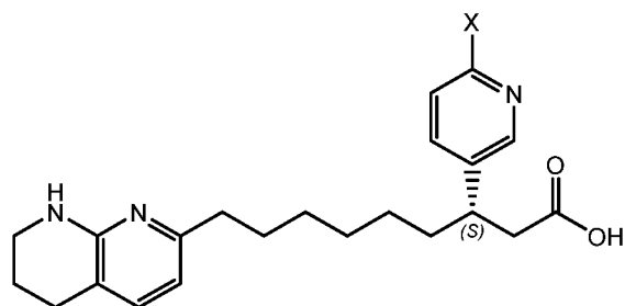
(Structure 29b),
