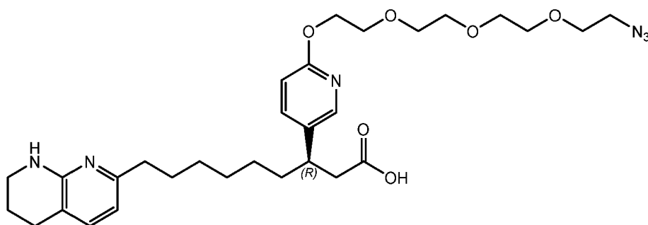
(Structure 28c).
