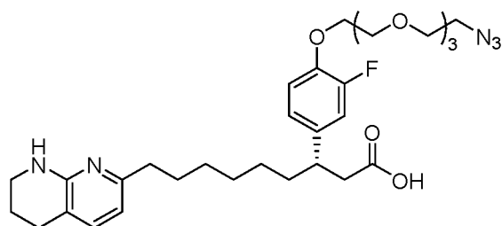
(Structure 31c).
