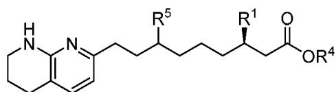
(Formula VII),
