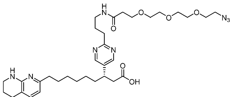
(Structure 39c).
