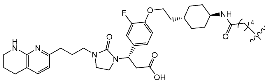
(Structure 2.3a);
