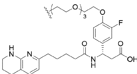
(Structure 37a);
