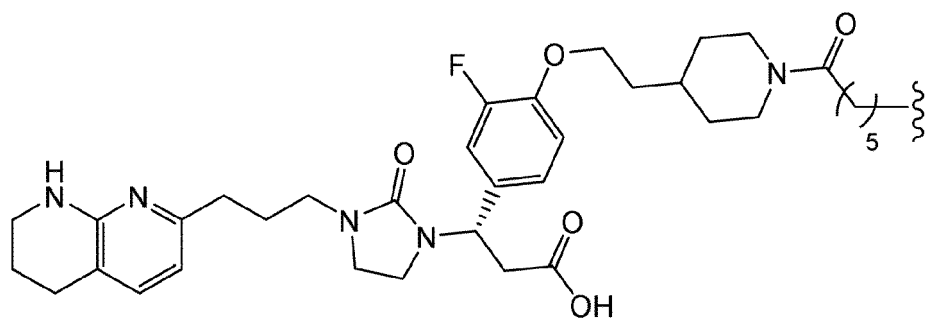
(Structure
