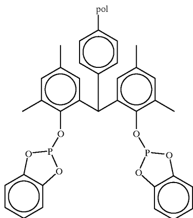
Supported Ligand SL56
