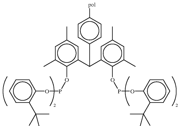
Supported Ligand SL60
