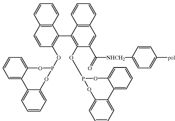
Supported Ligand SL23
