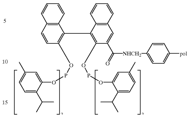
Supported Ligand SL24
