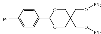
Supported Ligand SL3-1
