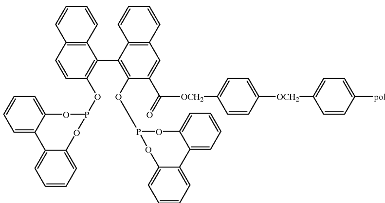
Supported Ligand SL28
