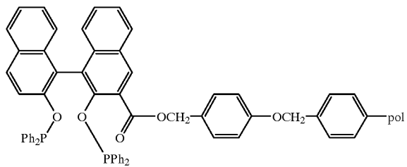
Supported Ligand SL29
