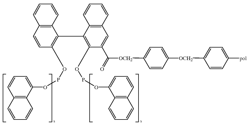
Supported Ligand SL32
