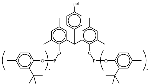
Supported Ligand SL61
