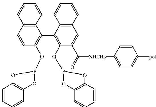
Supported Ligand SL27
