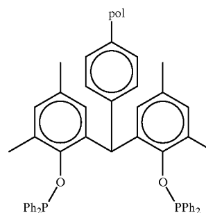
Supported Ligand SL55
