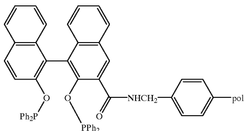
Supported Ligand SL26
