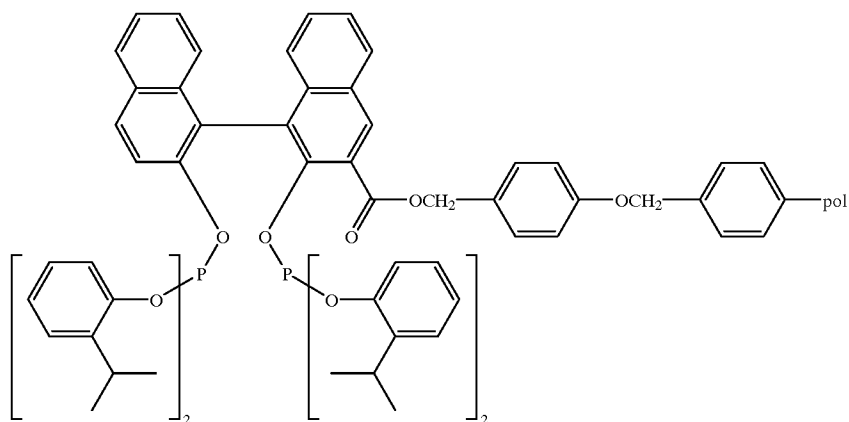
Supported Ligand SL31
