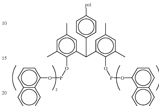
Supported Ligand SL54
