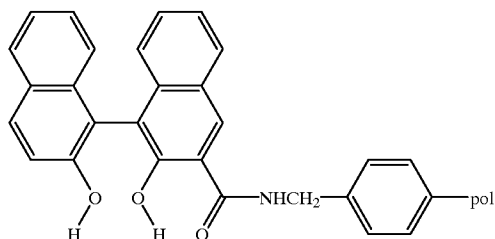
SD10 Supported diol SD10
