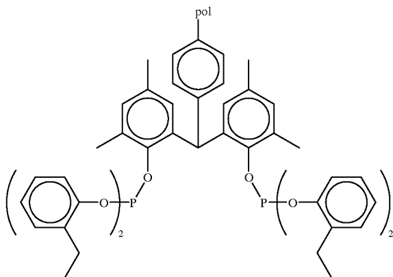
Supported Ligand SL57
