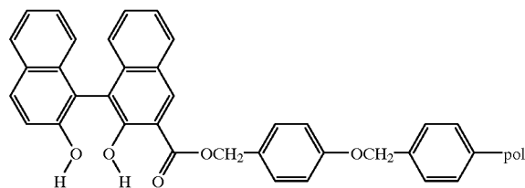
SD11 Supported Diol SD11
