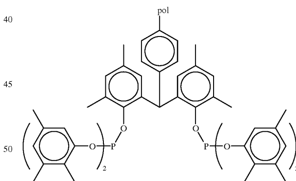
Supported Ligand SL59
