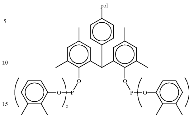
Supported Ligand SL58
