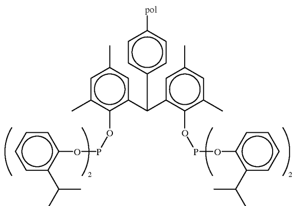
Supported Ligand SL52
