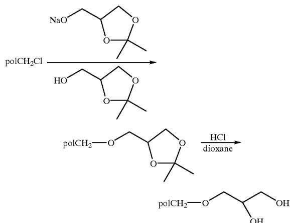
Supported diol SD6
