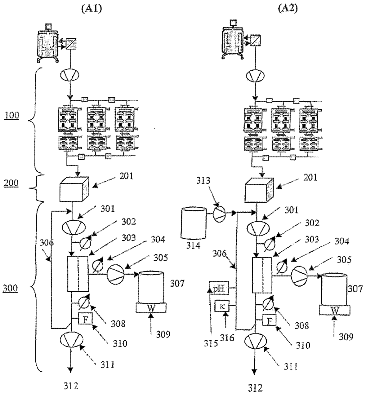
Figure 2: Schematic representation of 2 embodiments of inventive device A for continuous, integrated and sterile manufacturing. Schematic of embodiment A1 shown on left hand side and schematic of embodiment A2 shown on right hand side.
