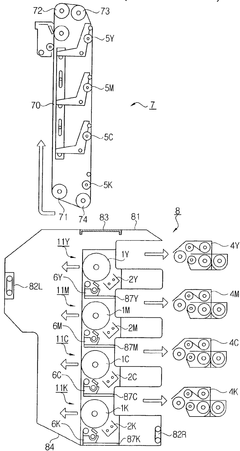
FIG. 5 (PRIOR ART)
