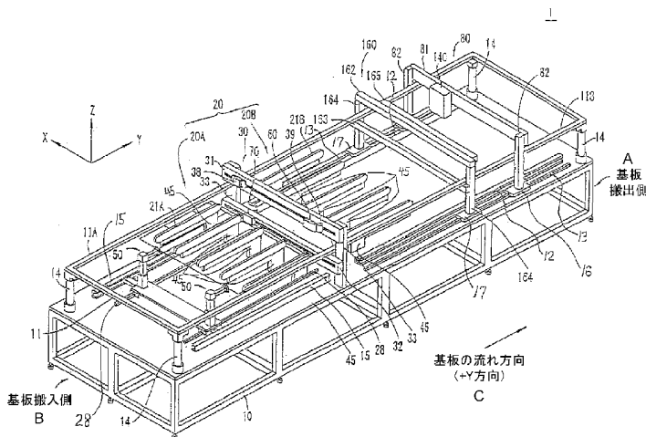
A... SUBSTRATE CARRY-OUT SIDE B... SUBSTRATE CARRY-IN SIDE C... DIRECTION OF SUBSTRATE FLOW (+Y DIRECTION)
