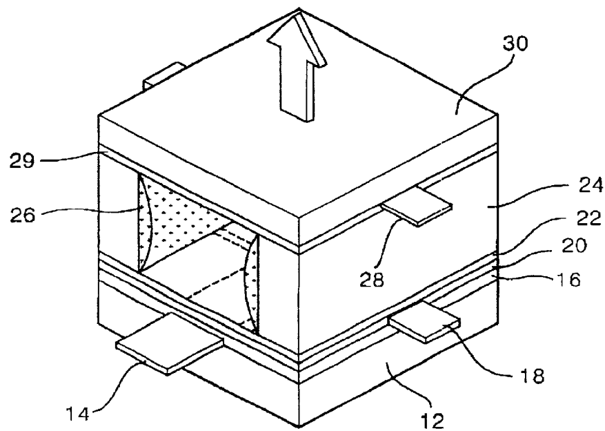
FIG. 2 RELATED ART
