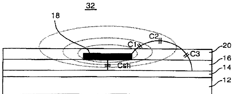
FIG. 3 RELATED ART
