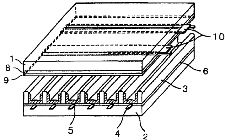
FIG. 2 RELATED ART
