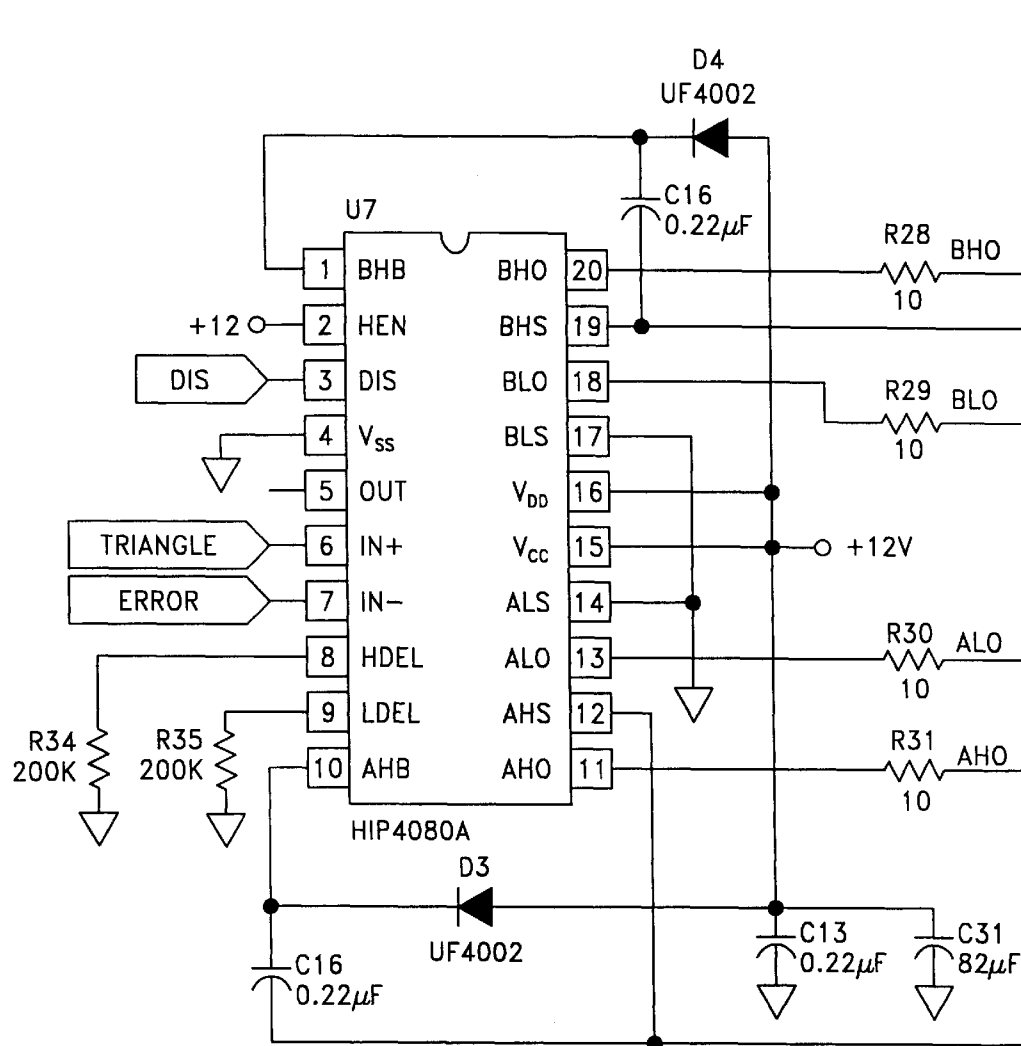
FIG. 2B-1 (PRIOR ART)
