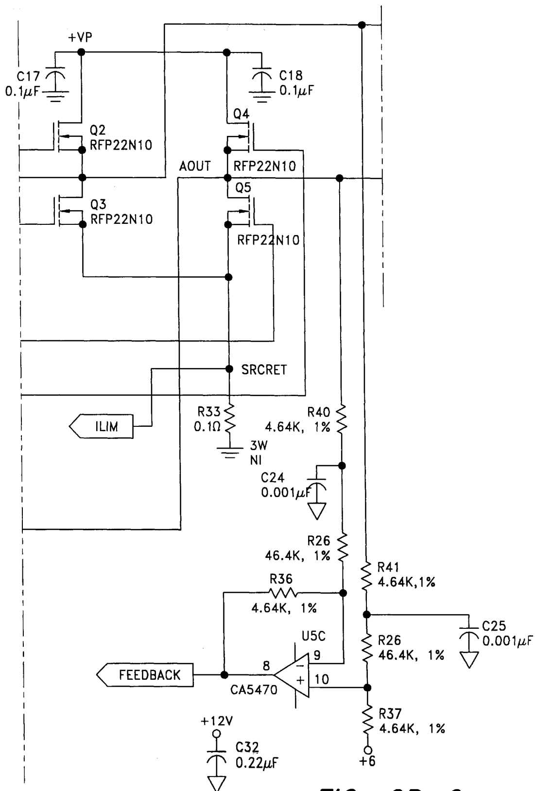
FIG. 2B-2 (PRIOR ART)
