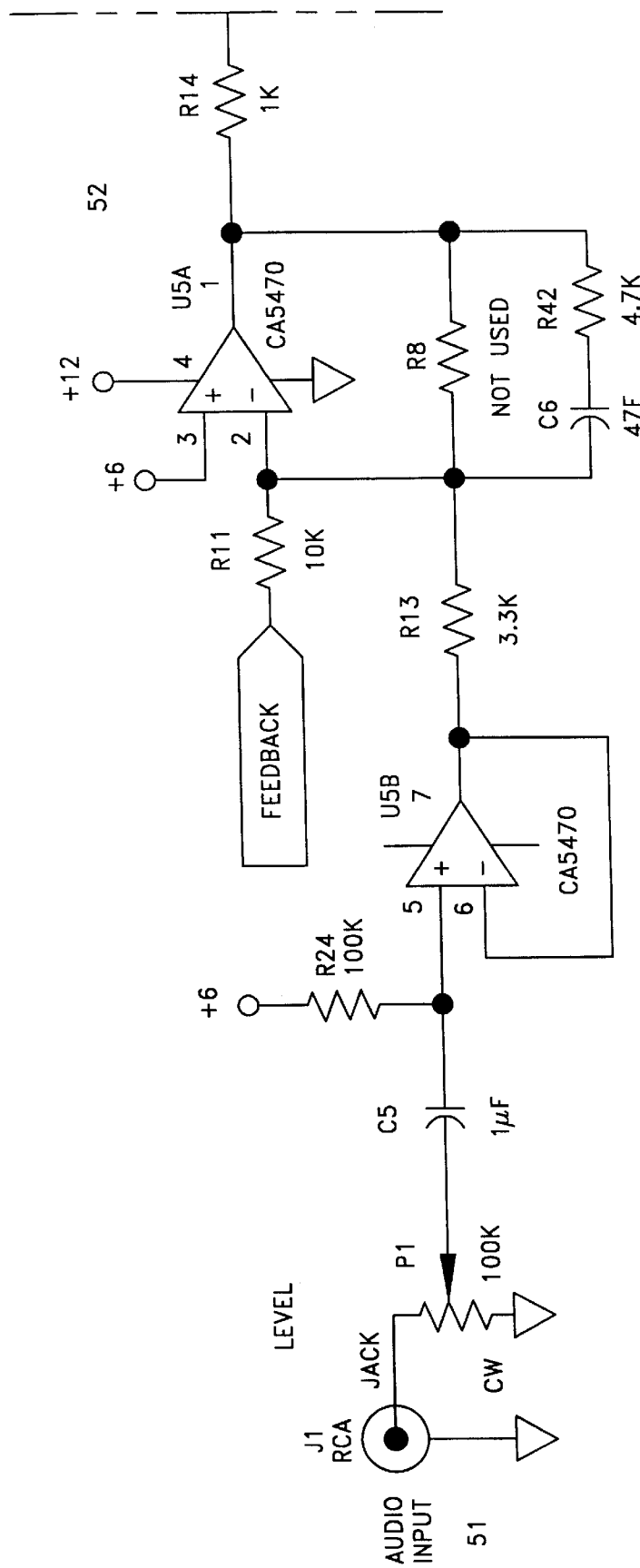
FIG. 2A-1 (PRIOR ART)
