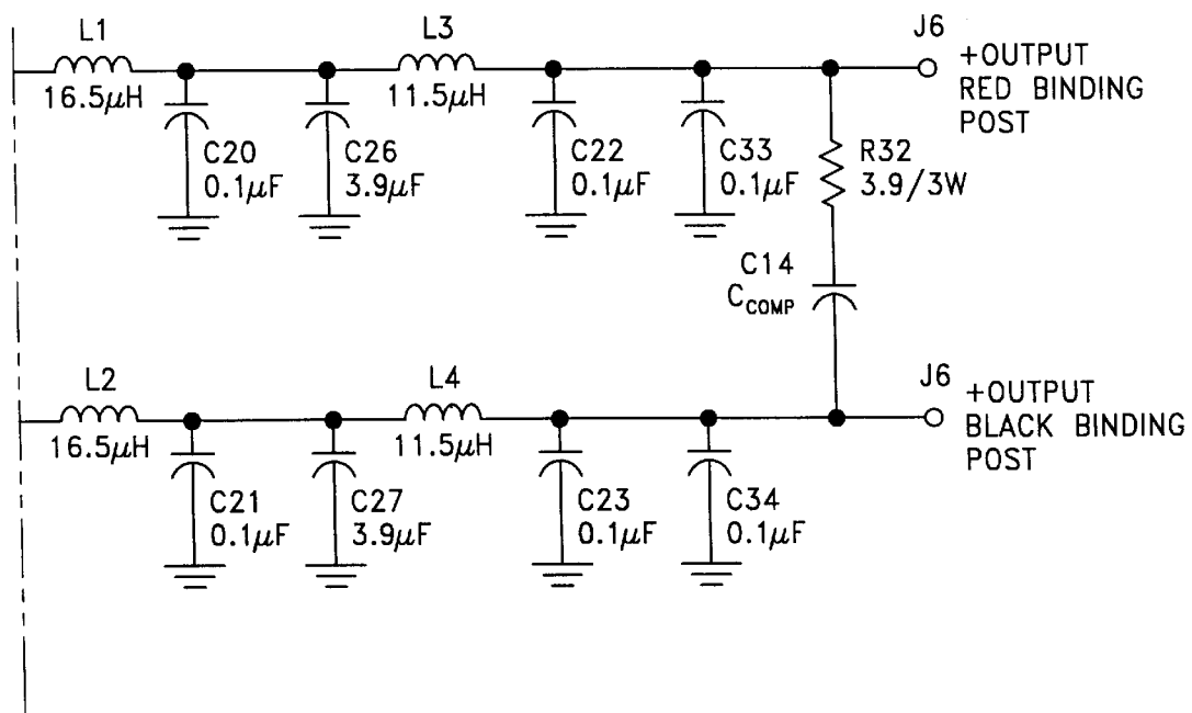
FIG. 2B-3 (PRIOR ART)
