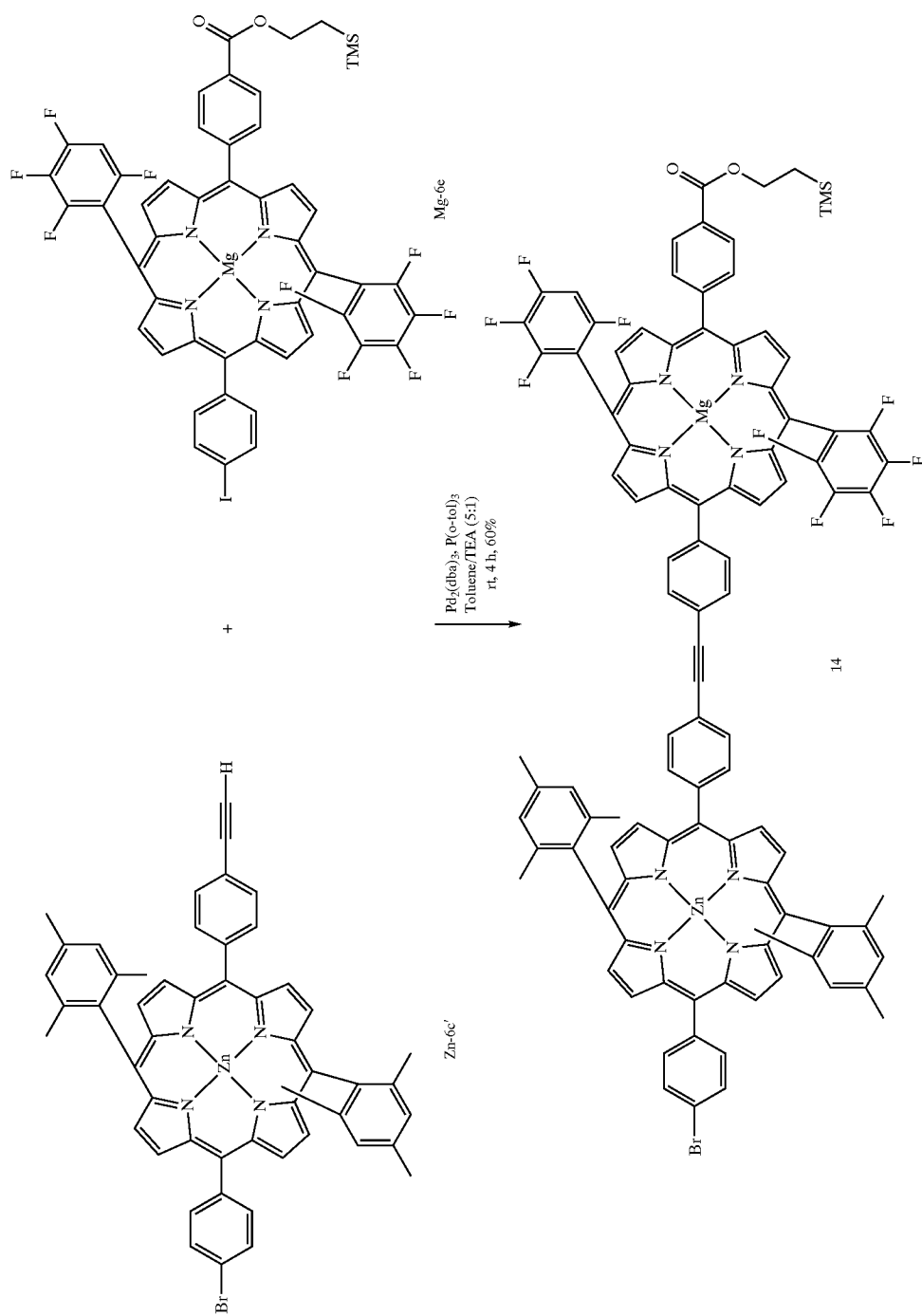
Scheme 17
