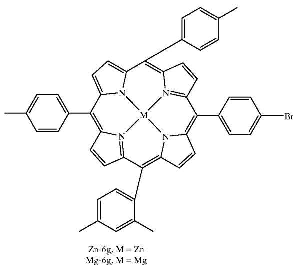
Scheme 14
