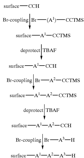
Scheme 10
