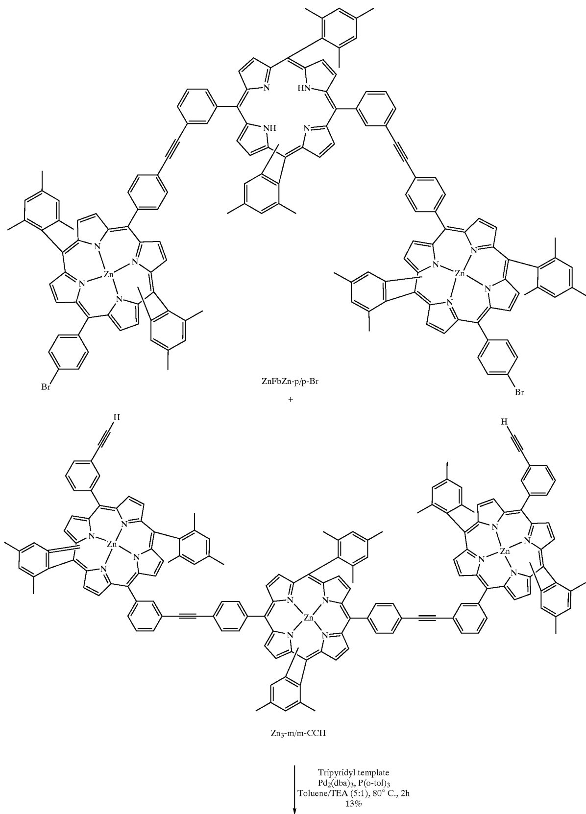
Scheme 24
