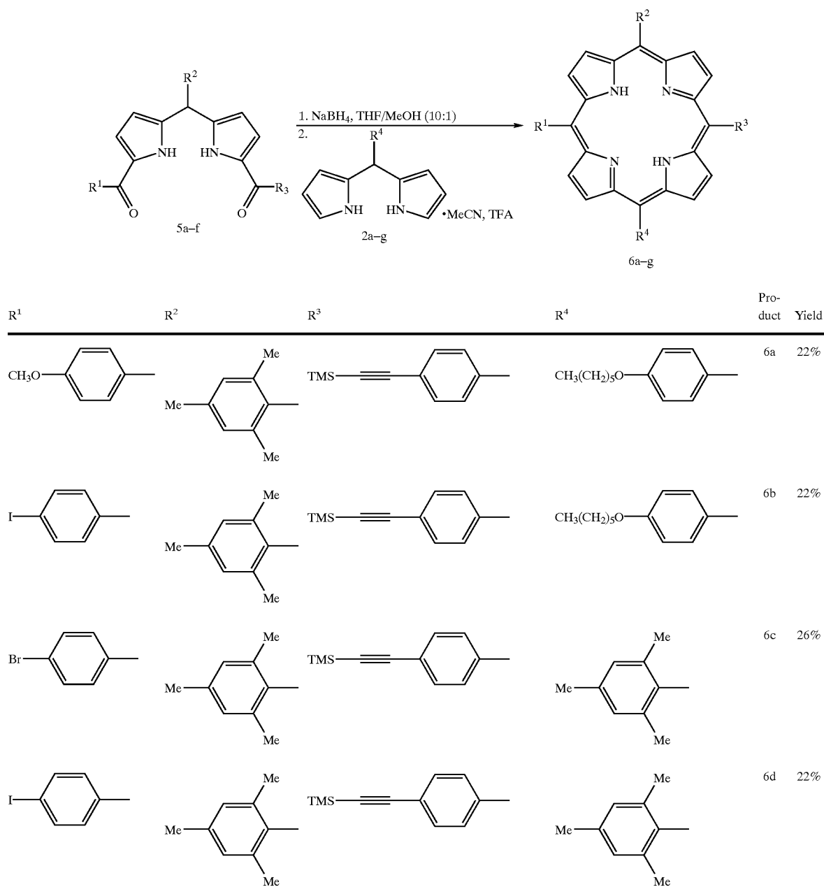
Scheme 12
