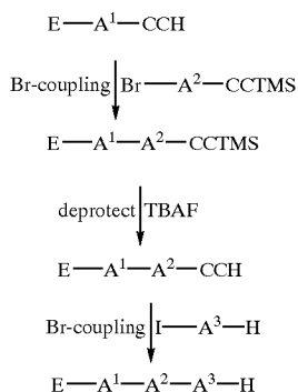
Scheme 8
