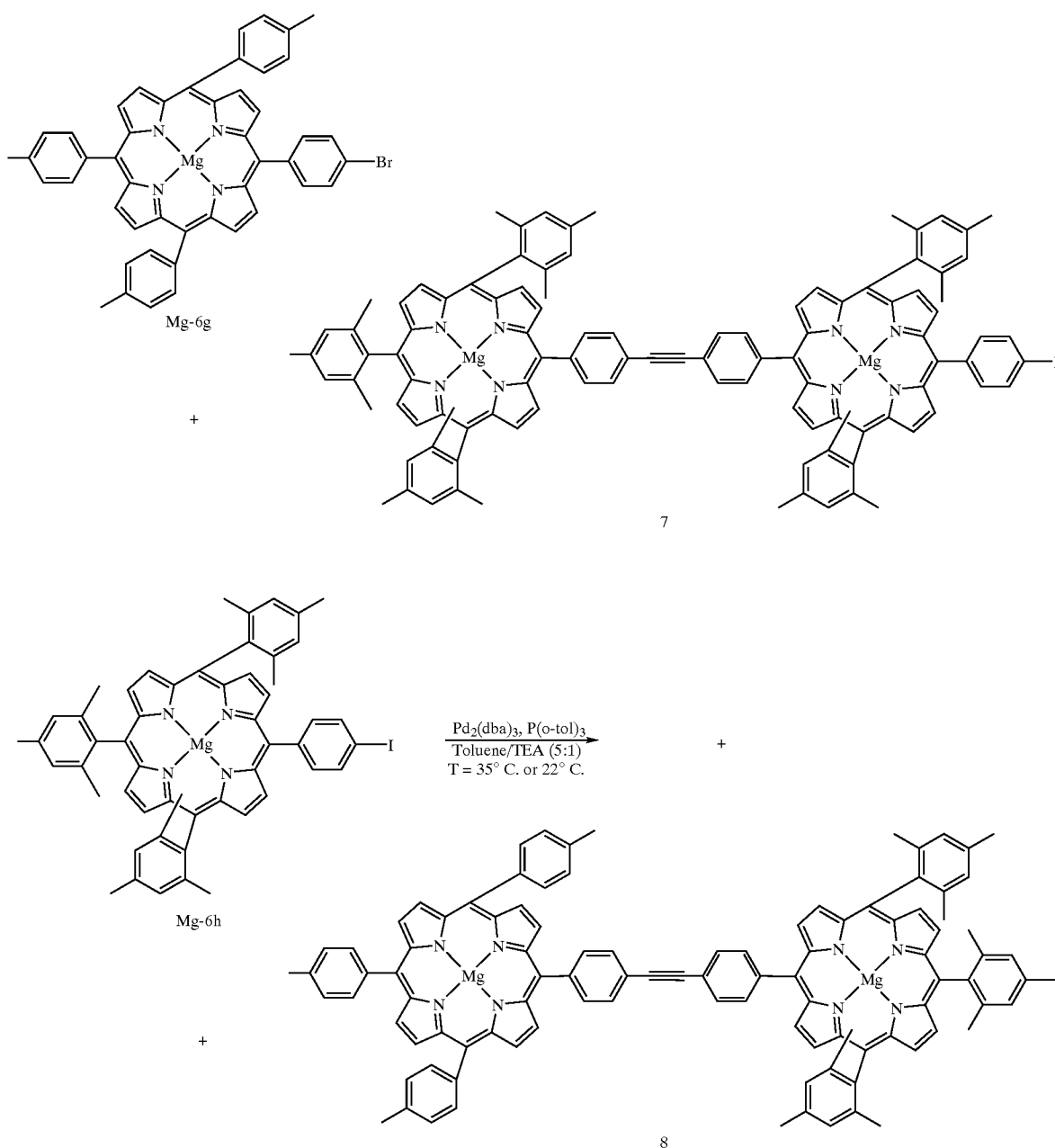
Scheme 13
