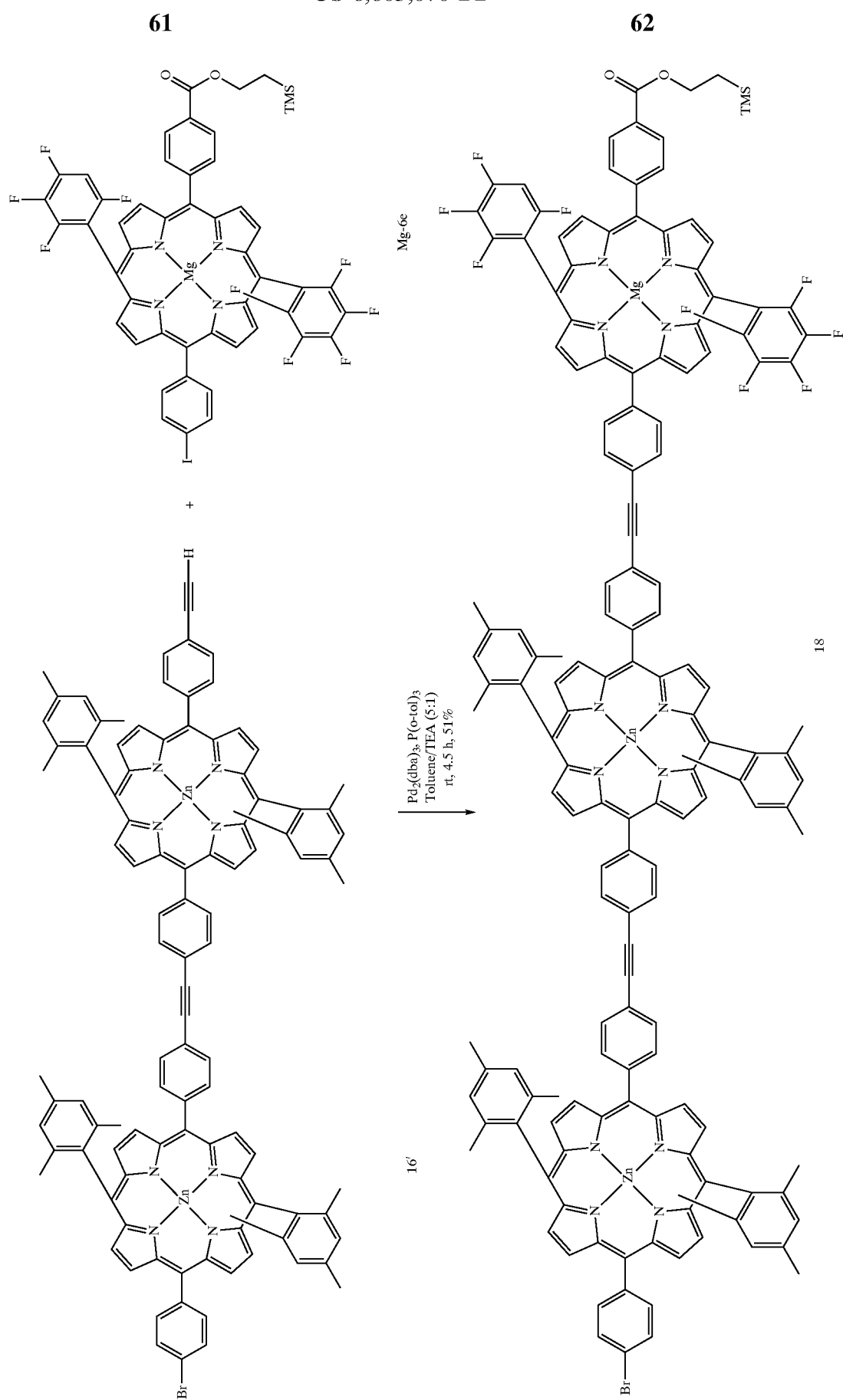
Scheme 19
