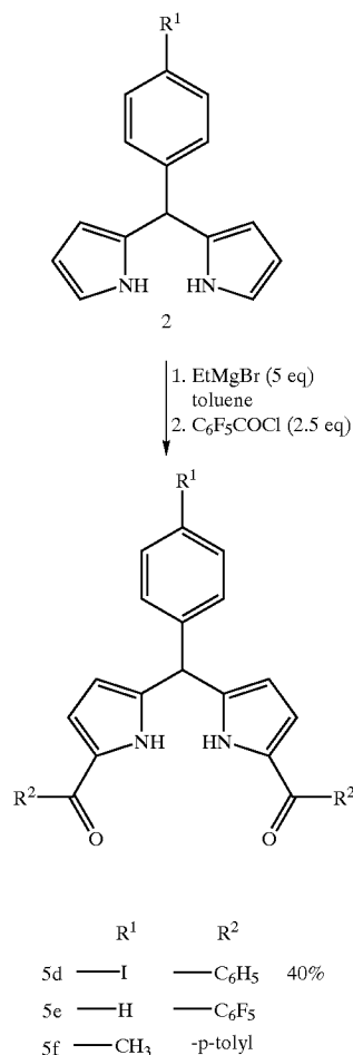
Scheme 11C
