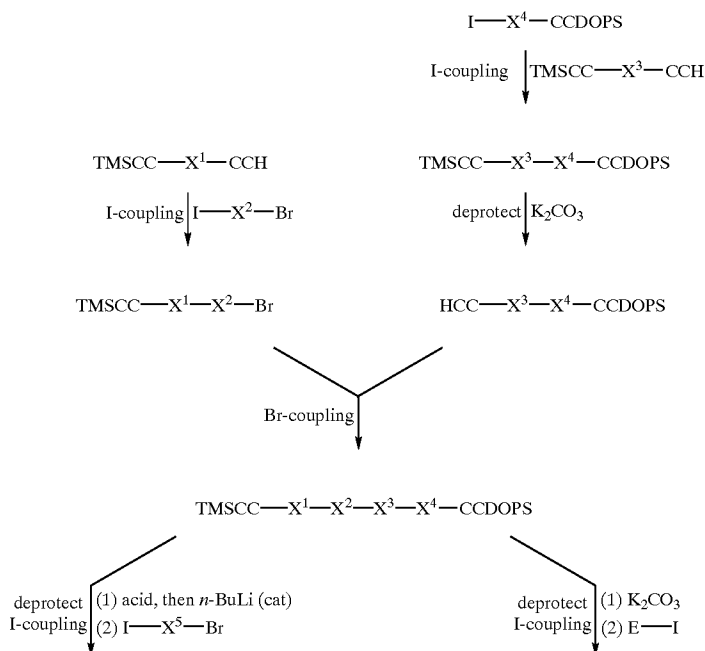
Scheme 7
