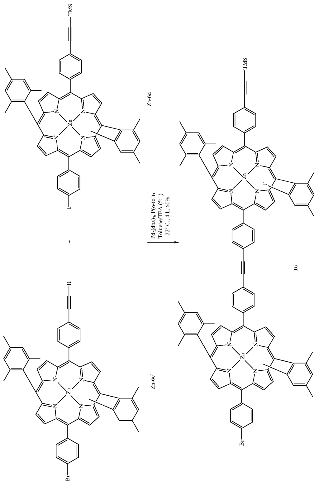
Scheme 18
