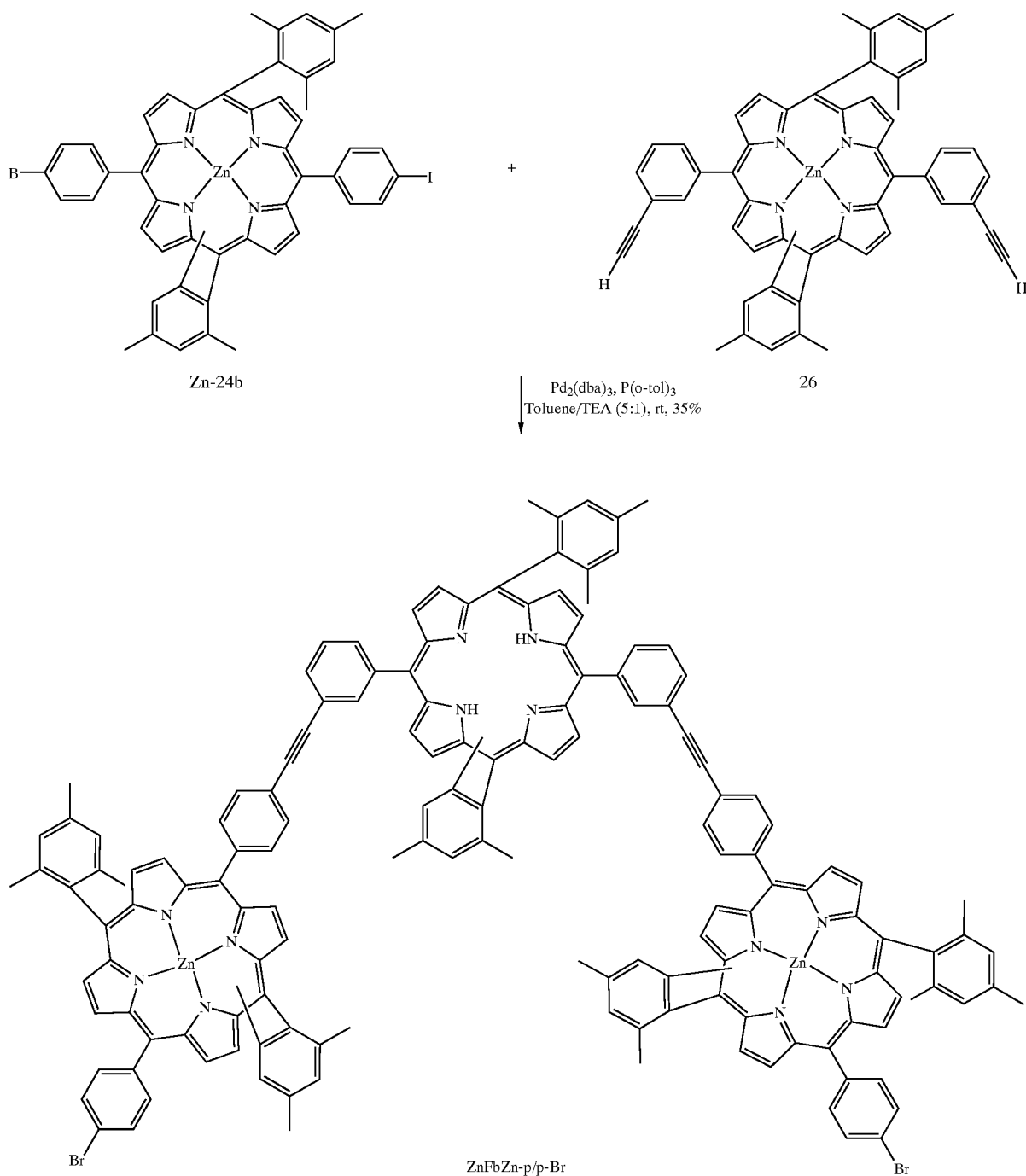
Scheme 23
