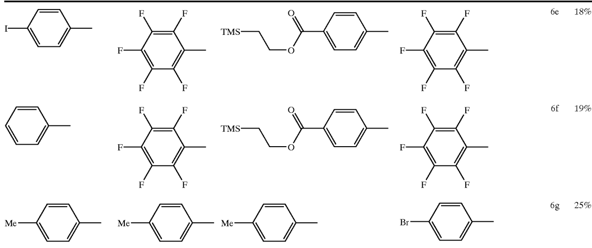
Scheme 12
