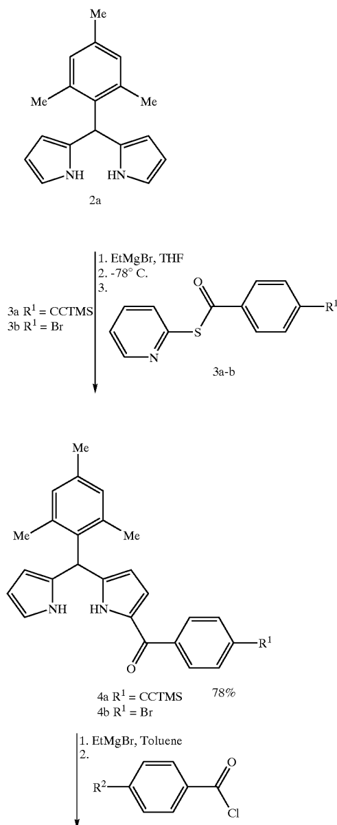
Scheme 11B
