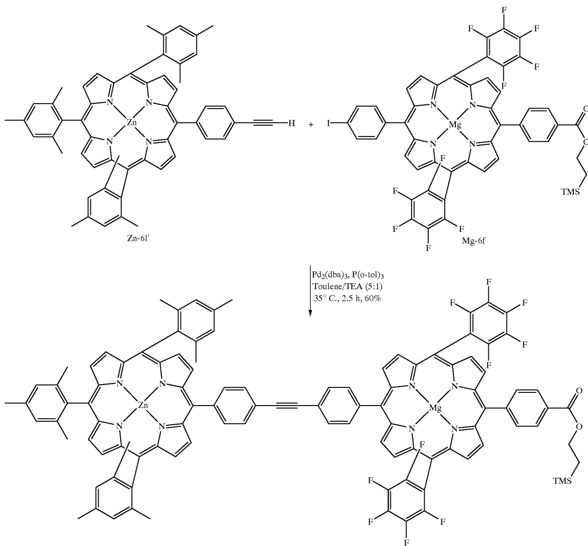
Scheme 20
