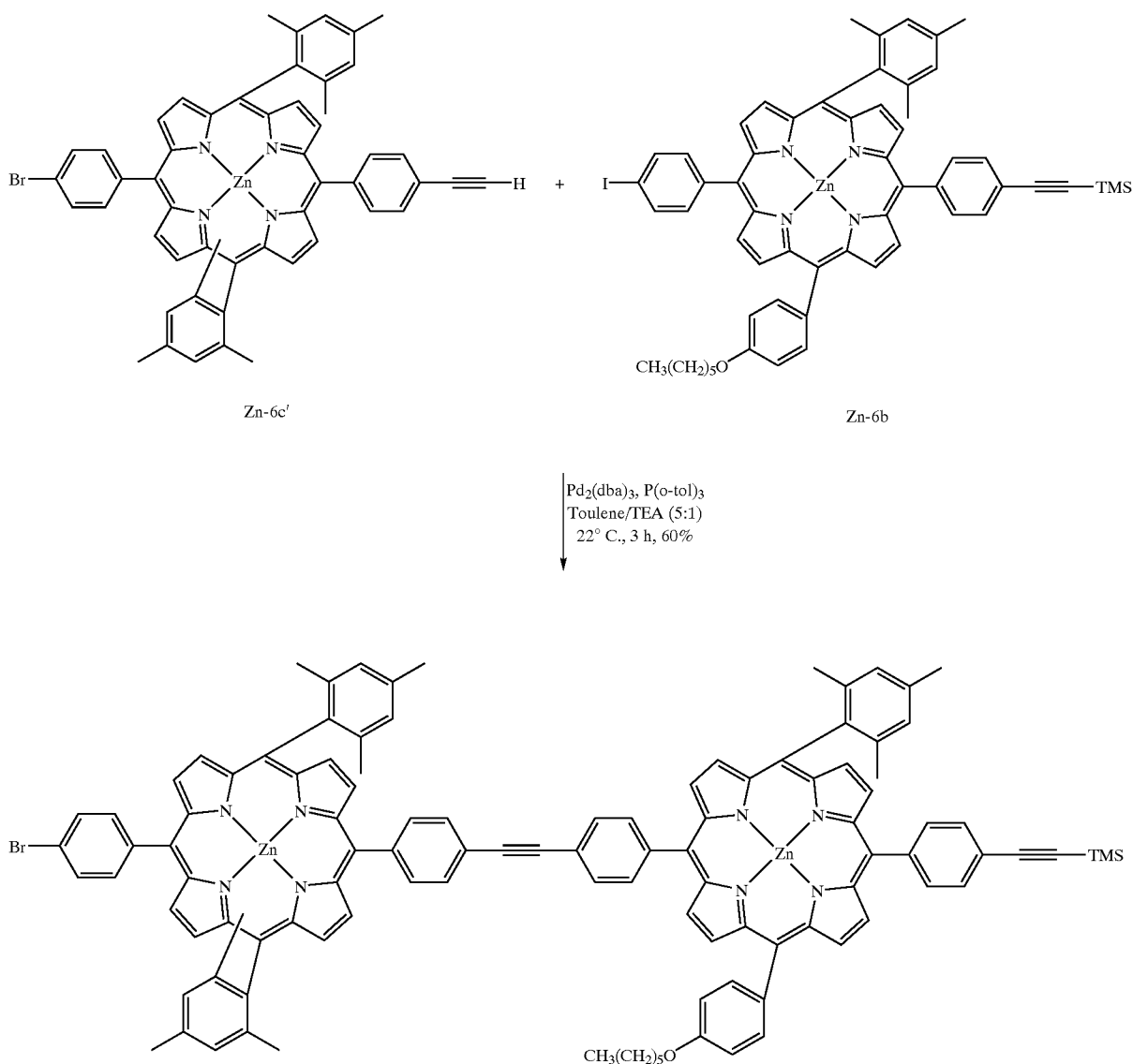
Scheme 15
