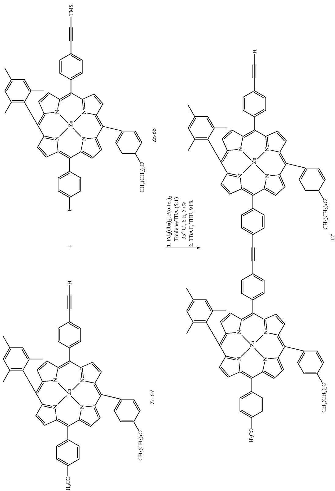
Scheme 16
