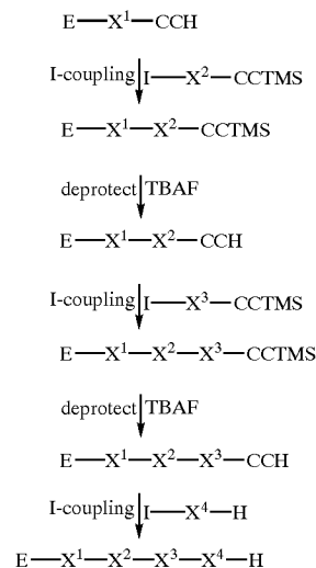
Scheme 1
