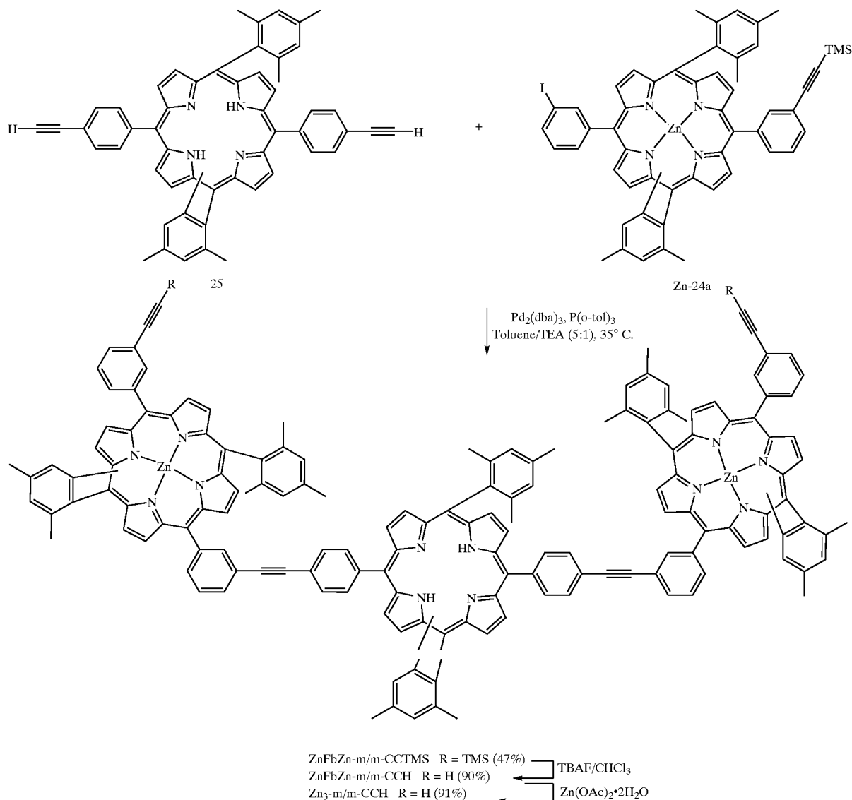
Scheme 22
