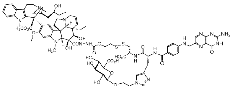
Conjugate of DAVLBH.
