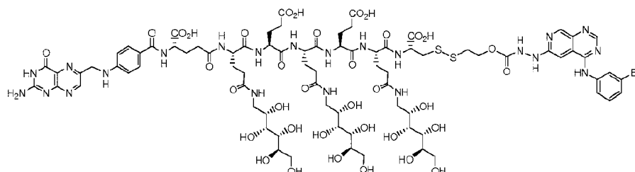
EC0640: Conjugate of 4-[(3-Bromophenyl)amino]-6-hydrazino-pyrido[3,4-d]pyrimidine
