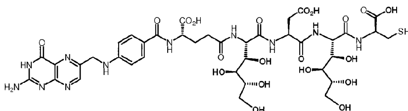
EC0244: \text{C}_{38}\text{H}_{51}\text{N}_{11}\text{O}_{20}\text{S} ; MW 1013.94; Exact Mass: 1013.30
