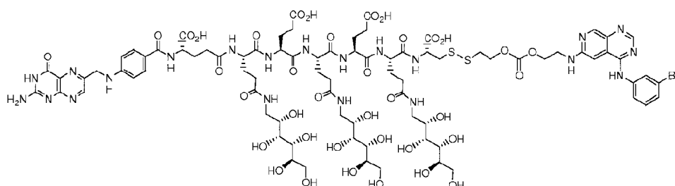
EC0631 Conjugate of the tyrosine kinase inhibitor 4-[(3-bromophenyl)amino]-6-[(2-hydroxyethyl-amino)-pyrido[3,4-d]pyrimidin-5-yl] group, C 83 H 114 BrN 21 O 37 S 2 , MW 2141.95, Exact Mass: 2139.63
