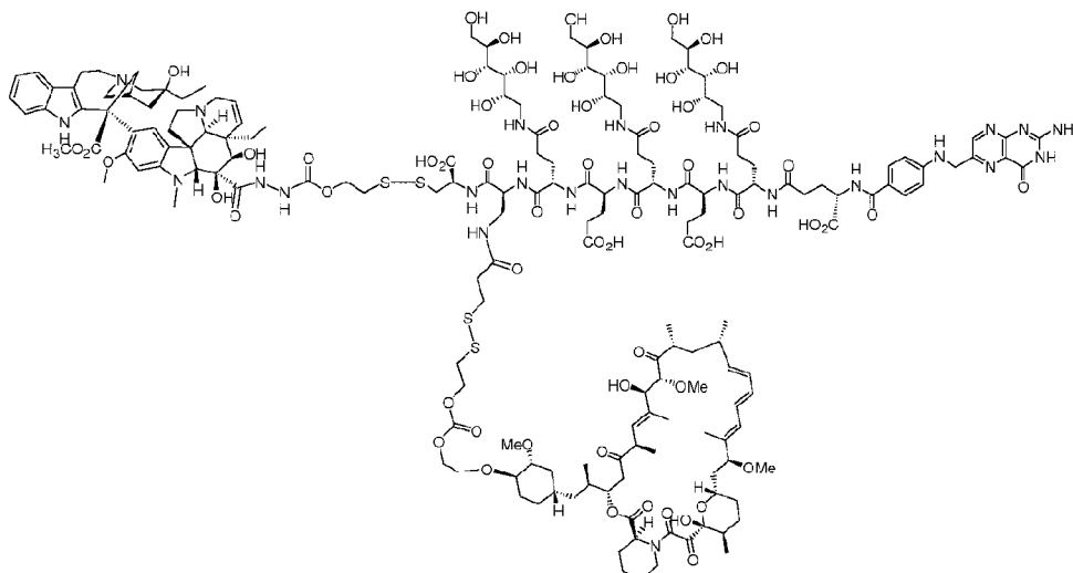
5 EC0636 Conjugate of DAVLBH and Everolimus. C 173 H 251 N 25 O 61 S 4 , MW 3785.23, Exact Mass: 3782.62
