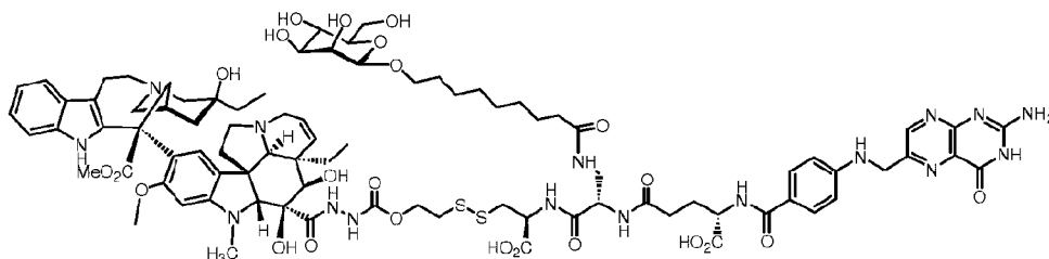
Conjugate of DAVLBII including a \beta -alkyl mannopyranoside.
