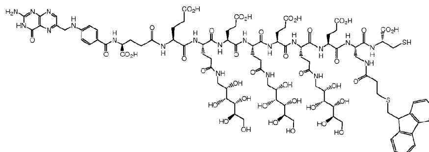
EC0559 Optionally selective multidrug intermediate for two drugs. C 90 H 121 N 19 O 36 S 3 , MW 2141.22, Exact Mass: 2139.74
