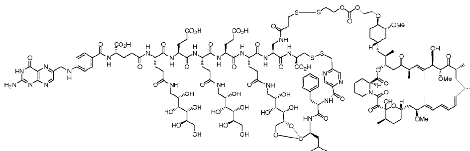
EC0582 Conjugate of Bortezomib and Everolimus. C 147 H 214 BN 23 O 54 S 4 , C, 53.40; H, 6.52; B, 0.33; N, 9.74; O, 26.13; S, 3.88, MW 3306.47, Exact Mass: 3304.37
