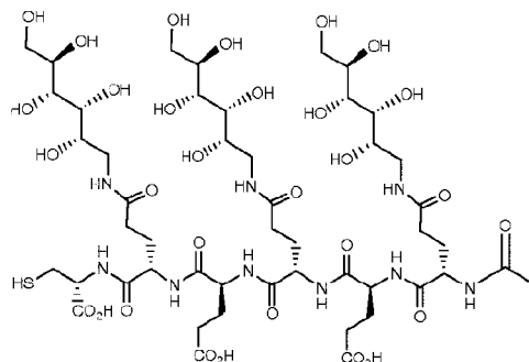
EC0586 Intermediate for optional non-target delivery. C 48 H 83 N 9 O 30 S, MW 1298.28, Exact Mass: 1297.50
