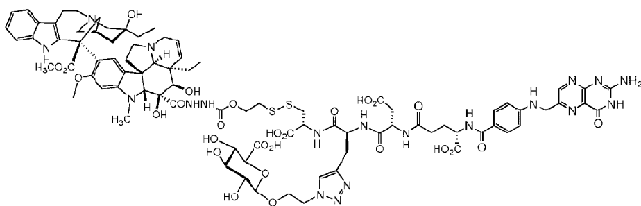
Conjugate of DAVLBH.
