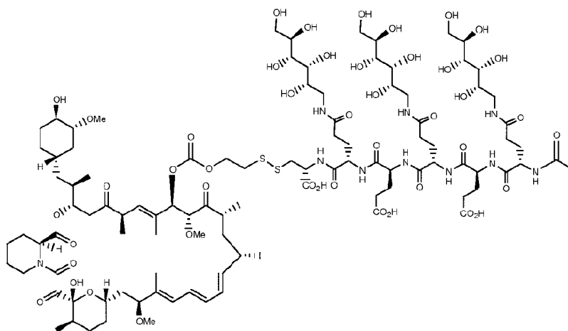
EC0591 Rapamycin conjugate intermediate for optional non-targeted delivery. C 102 H 164 N 10 O 45 S 2 , C, 52.93; H, 7.14; N, 6.05; O, 31.11; S, 2.77, MW 2314.57, Exact Mass: 10 2313.03
