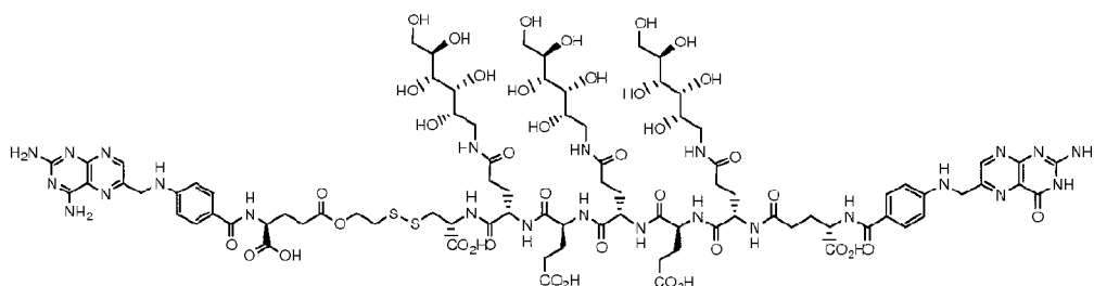
5 EC0551 Conjugate of aminopterins. C 86 H 120 N 24 O 39 S 2 , C, 47.42; H, 5.55; N, 15.43; O, 28.65; S, 2.94, MW 2178.14, Exact Mass: 2176.76
