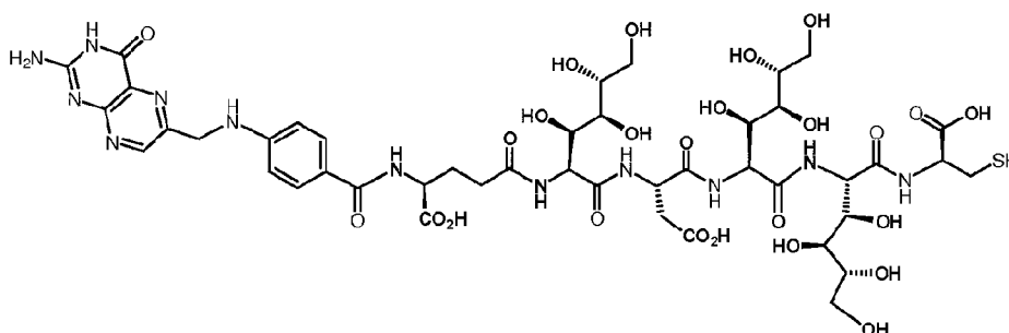
EC0257: \text{C}_{44}\text{H}_{62}\text{N}_{12}\text{O}_{25}\text{S} ; MW 1191.09; Exact Mass: 1190.37
