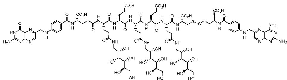
EC0544 Conjugate of cysteine analog of aminopterins. C 83 H 116 N 24 O 37 S 2 , C, 47.33; H, 5.55; N, 15.96; O, 28.11; S, 3.05, MW 2106.08, Exact Mass: 2104.74
