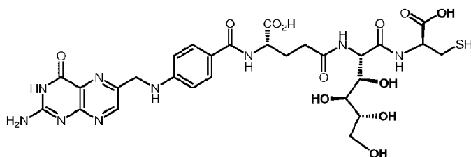
EC0233: \text{C}_{28}\text{H}_{35}\text{N}_9\text{O}_{12}\text{S} ; MW 721.70; Exact Mass: 721.21
