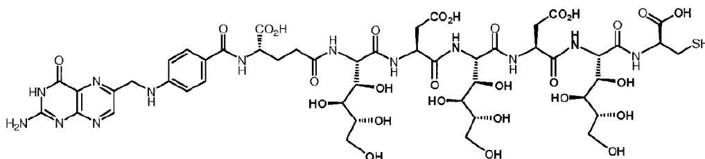
EC0261: \text{C}_{48}\text{H}_{67}\text{N}_{13}\text{O}_{28}\text{S} ; MW 1306.18; Exact Mass: 1305.39
