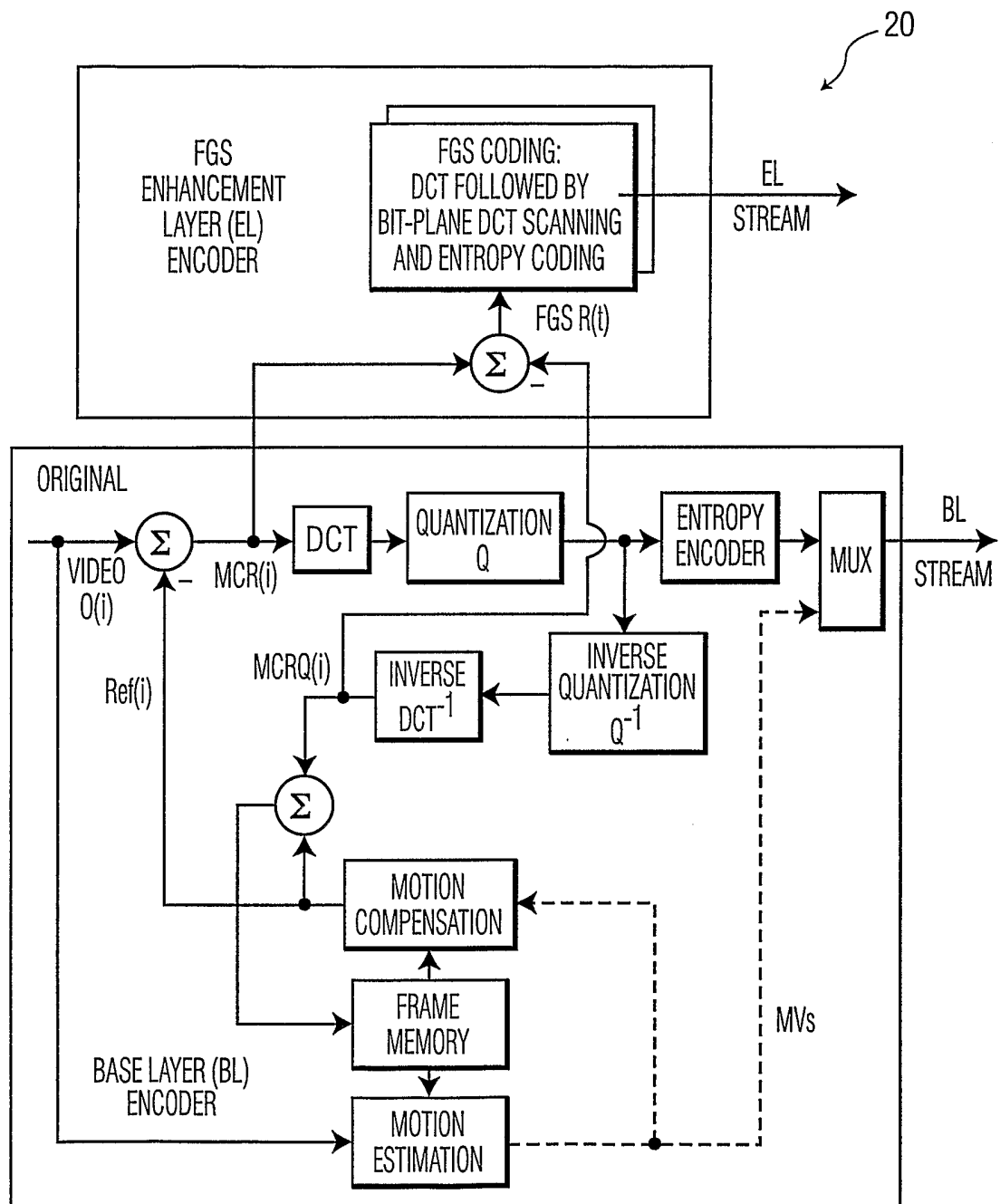
FIG. 2 (PRIOR ART)
