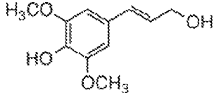
sinapyl alcohol
