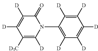
d 11 -5-Methyl-1-phenyl-1H-pyridin-2-one
