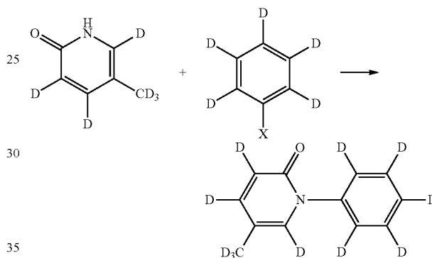
d 11 -5-Methyl-1-phenyl-1H-pyridin-2-one
