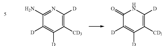
d 6 -5-Methyl-1H-pyridin-2-one
