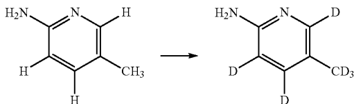
d 6 -5-methyl-pyridin-2-ylamine
