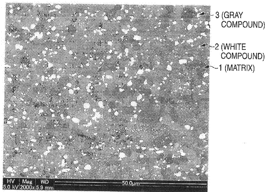
SEM PHOTOGRAPH
