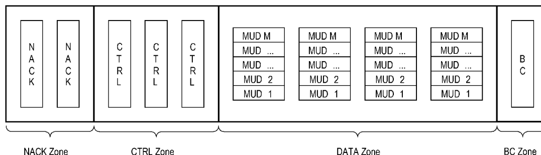
DIMA MAC Frame Structure
