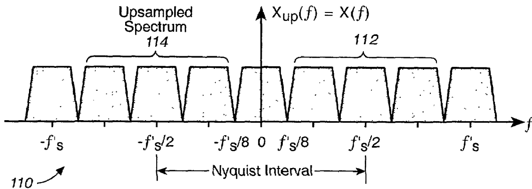
FIG._7 (PRIOR ART)
