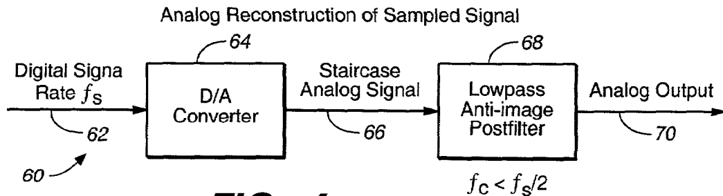
60 FIG. 4 (PRIOR ART)
