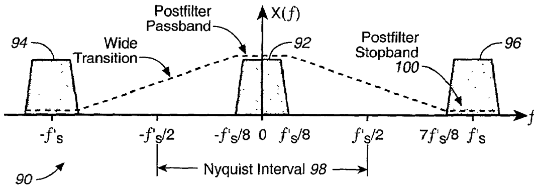
FIG._6 (PRIOR ART)
