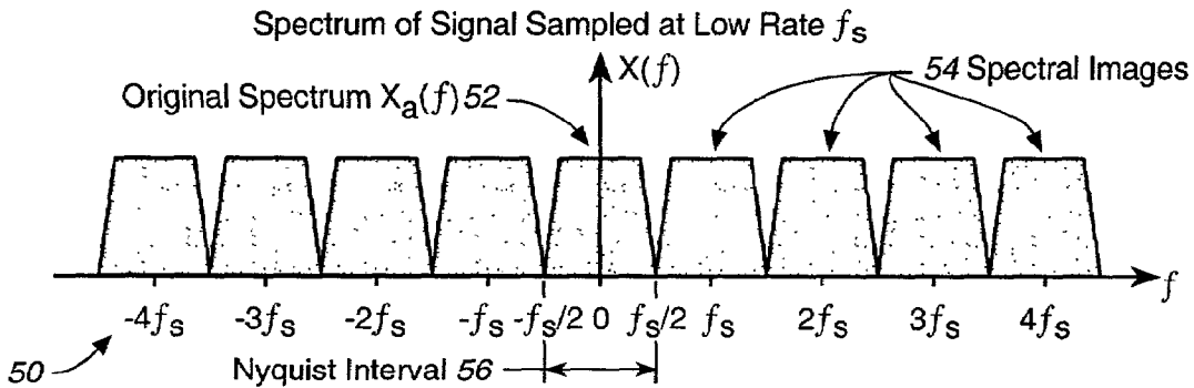
50 FIG. 3 (PRIOR ART)
