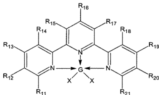
Formel (II)
