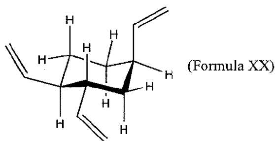
Isomer B
