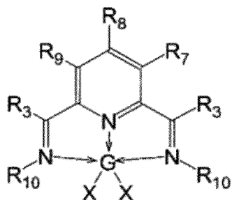
Formel (I)
