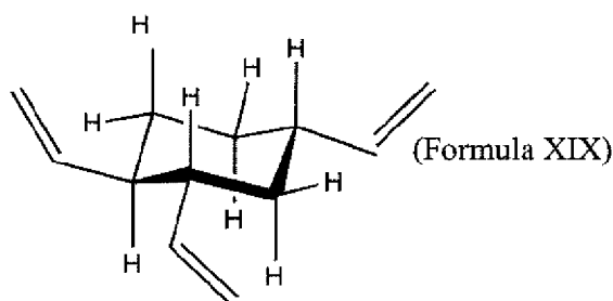
Isomer A
