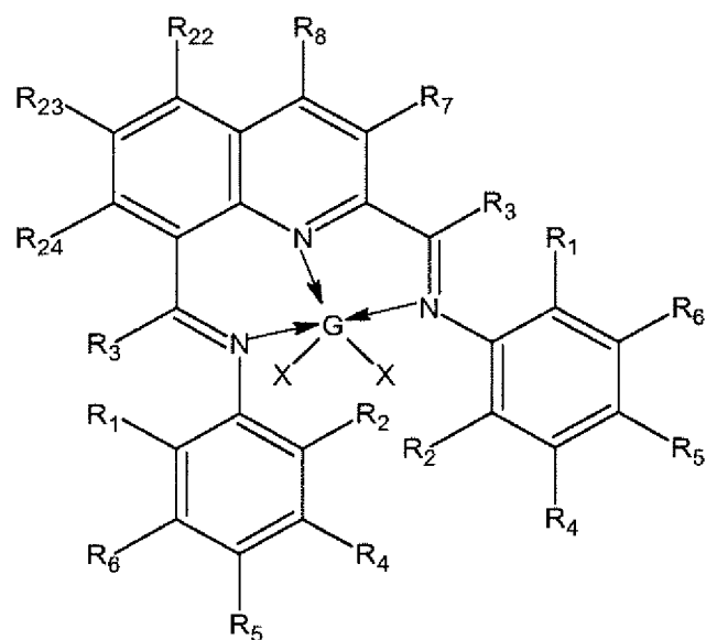
Formula (III)
