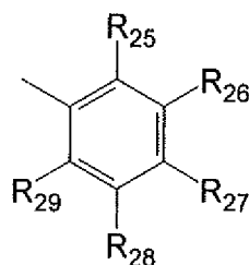
Formula (XXI)
