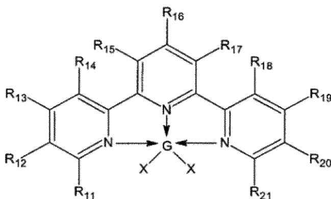
Formel (II)
