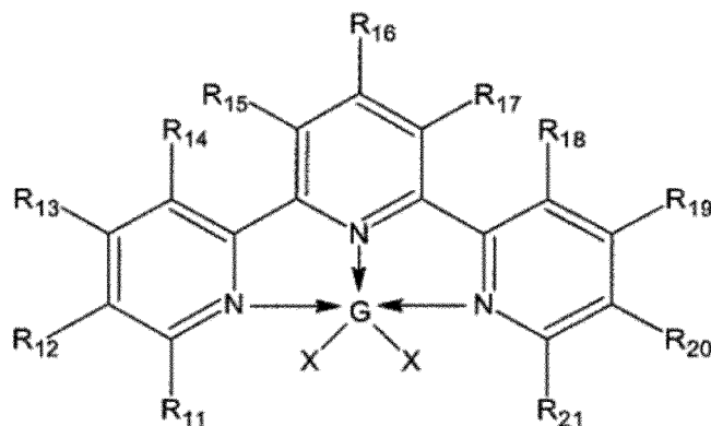
Formel (II)
