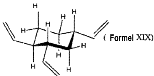
Isomer A
