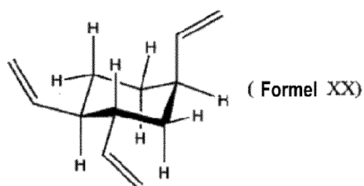
Isomer B
