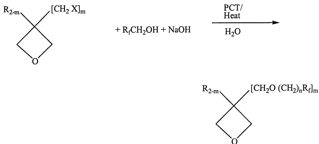
FOX Monomer
