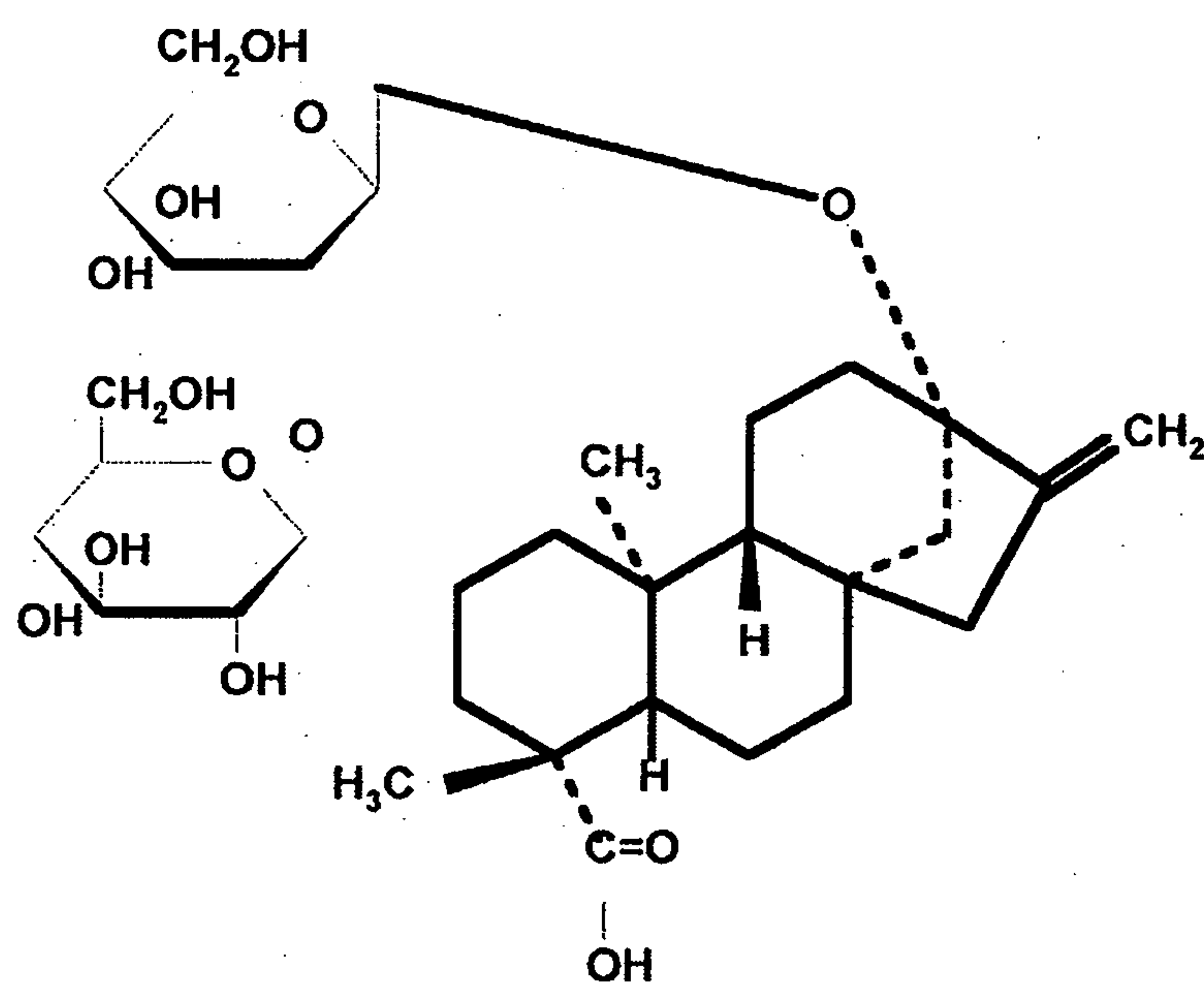
Steviolbioside
