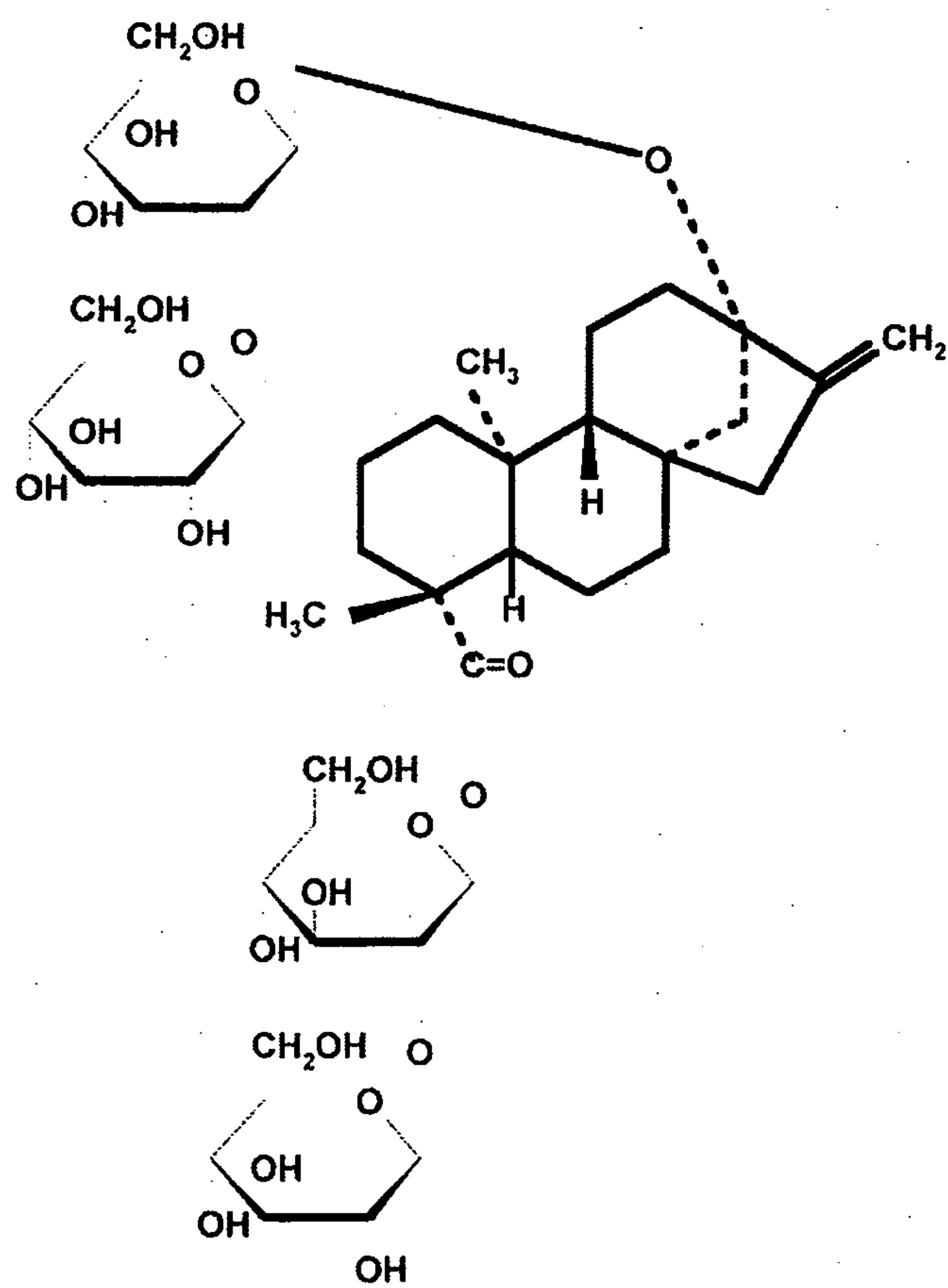
Rebaudioside E
