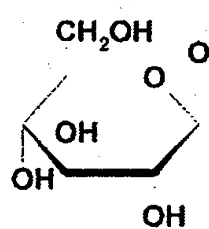
Rebaudioside A
