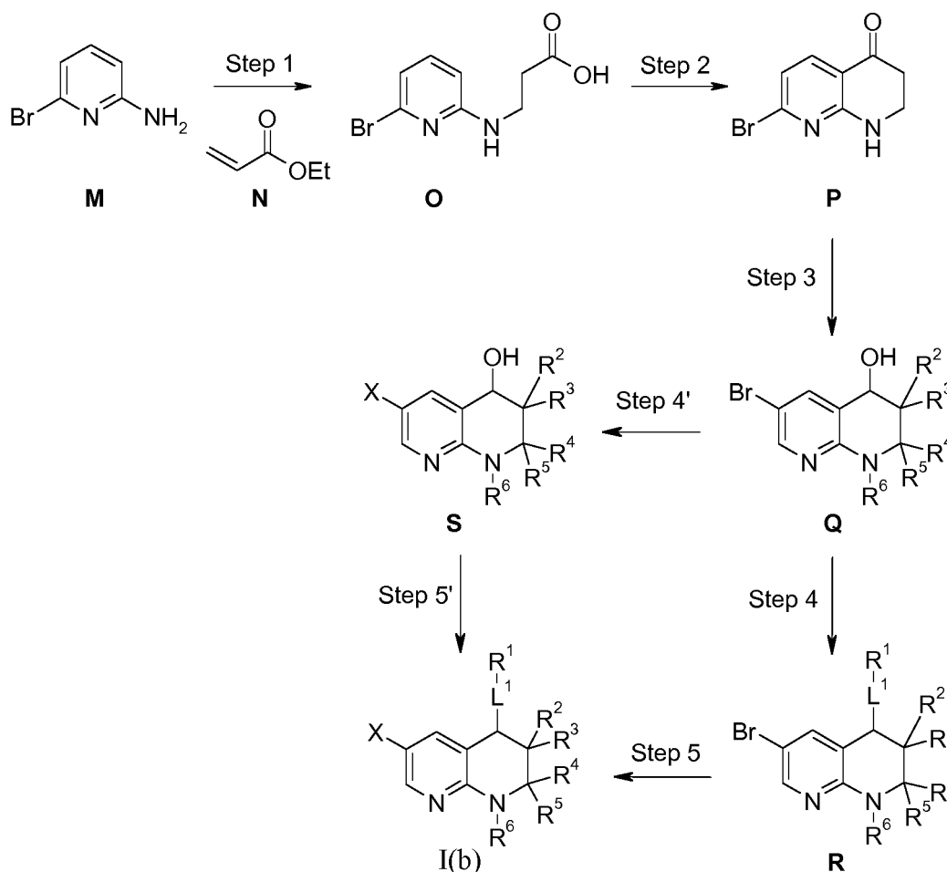
Scheme 5. Overall Synthesis: A = Carbon
