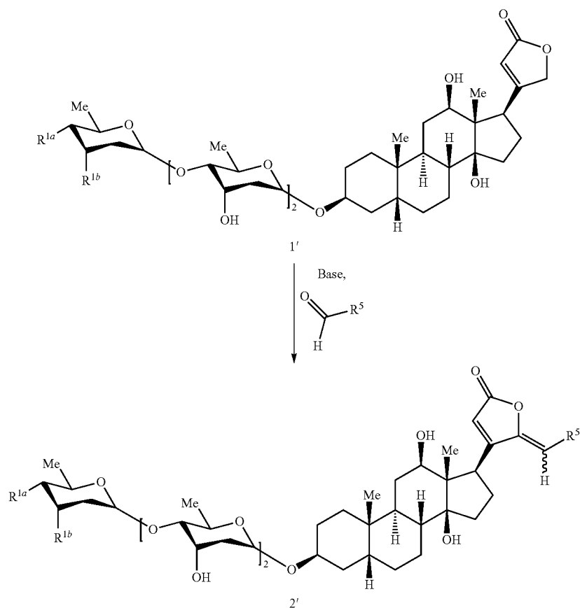
Scheme 2
