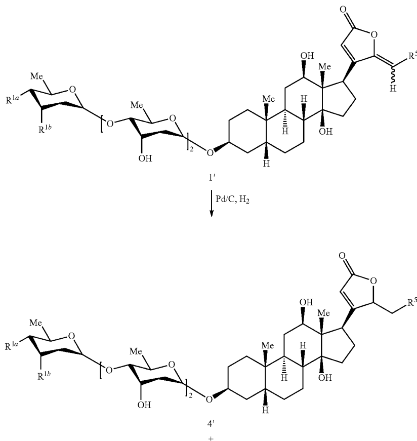
Scheme 4
