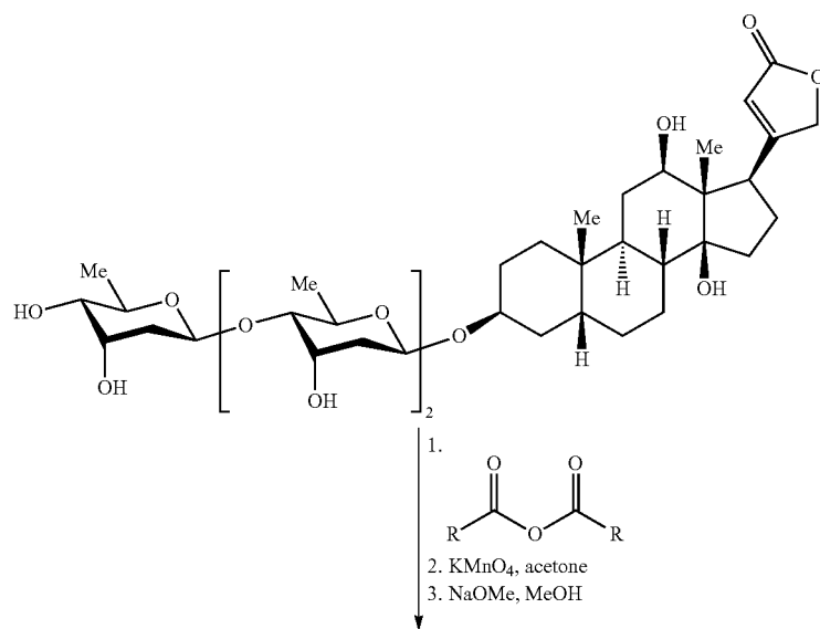
Scheme 5
