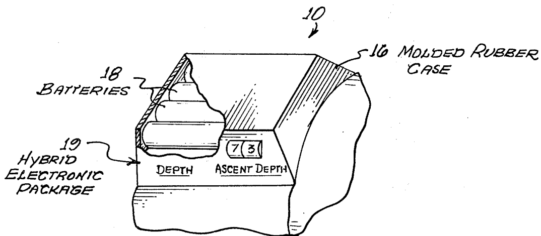
Fig. 2. MAIN COMPONENTS OF DECOMETER
