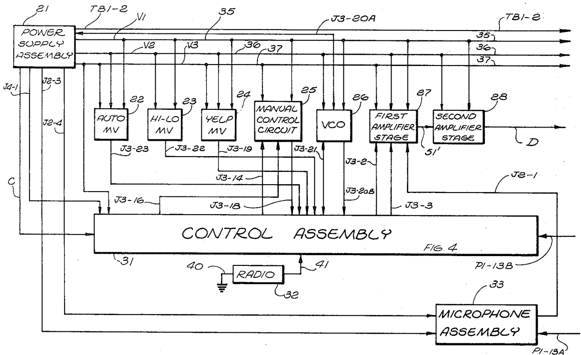
SOUND COMMUNICATION SYSTEM 20
