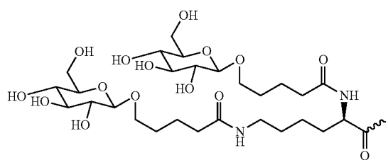
Formula XVIII
