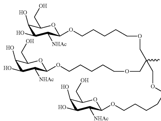
Formula VIII
