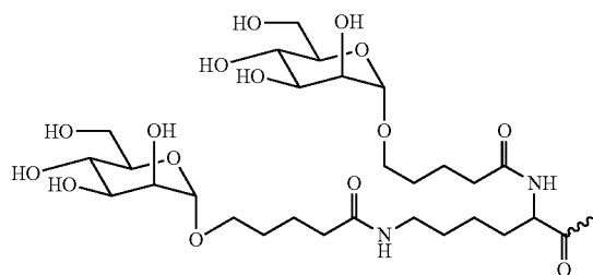
Formula XX
