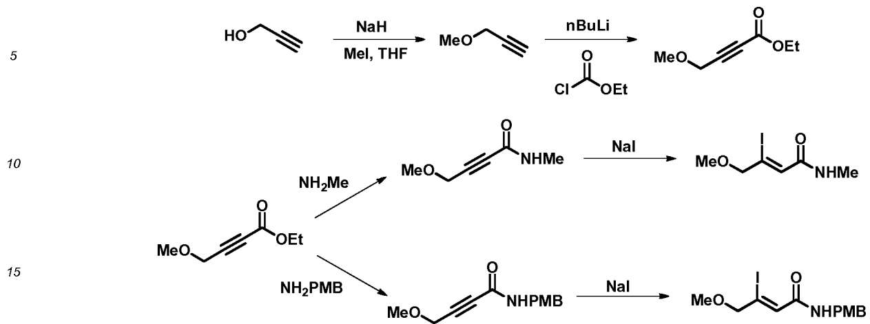
Scheme 7.2. Preparation of DNQ-P2 and DNQ-P3 Intermediates.
