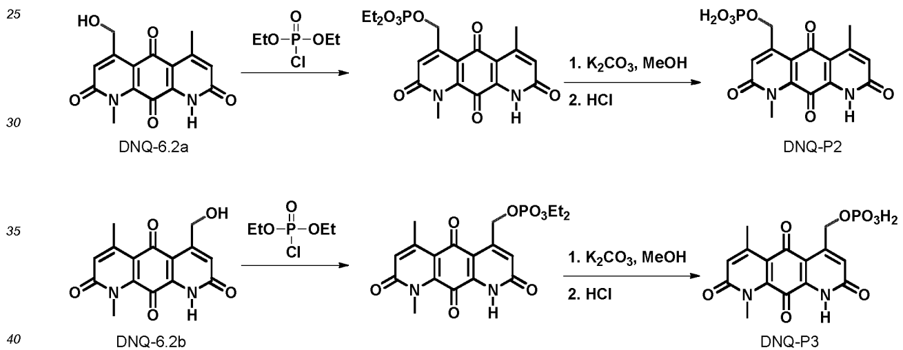
Scheme 7.3. Preparation of DNQ-P2 and DNQ-P3.
