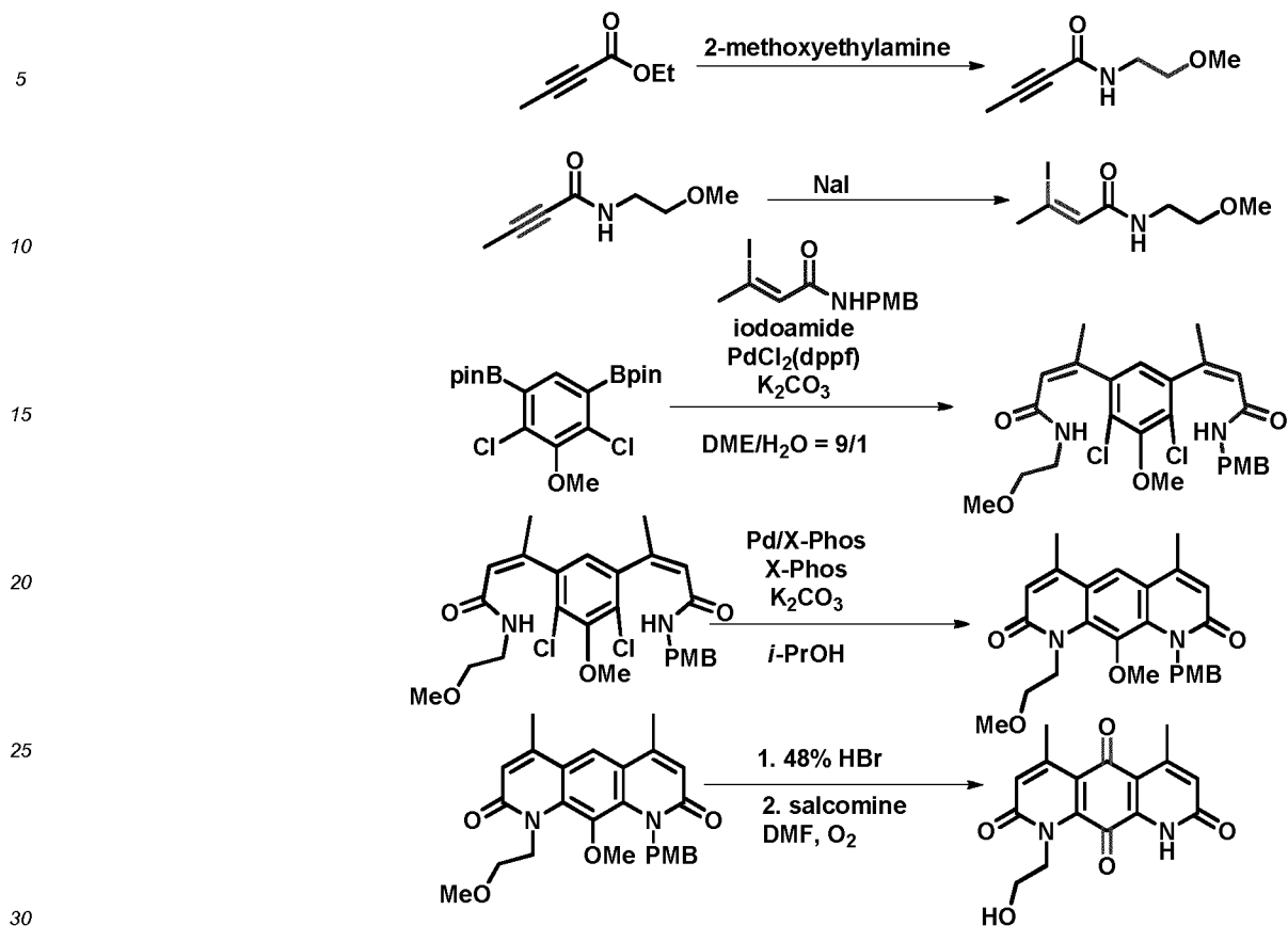
Scheme 7.4. Preparation of DNQ-P4.
