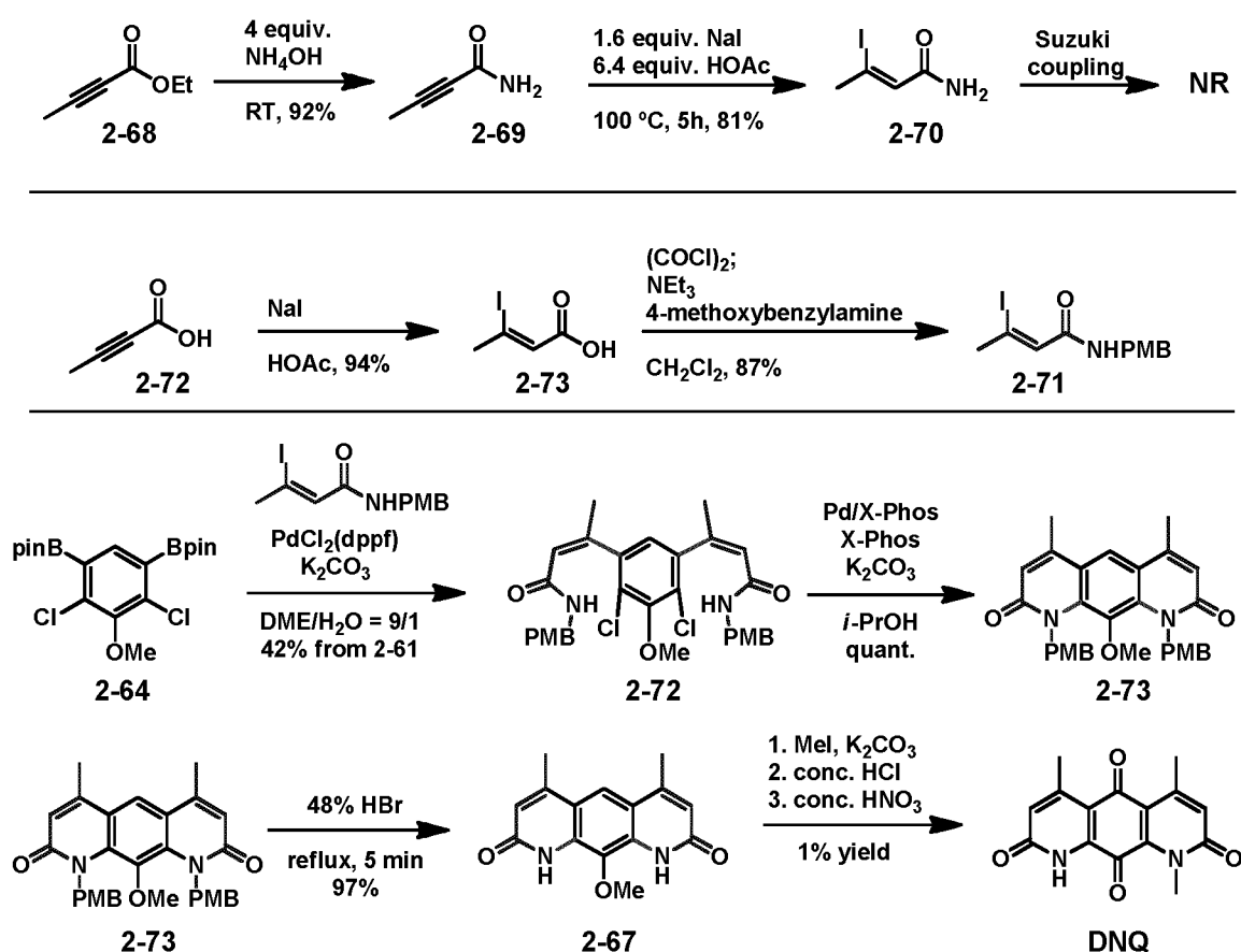
Scheme 1.13. Synthesis of DNQ by methylation of 2-67 .
