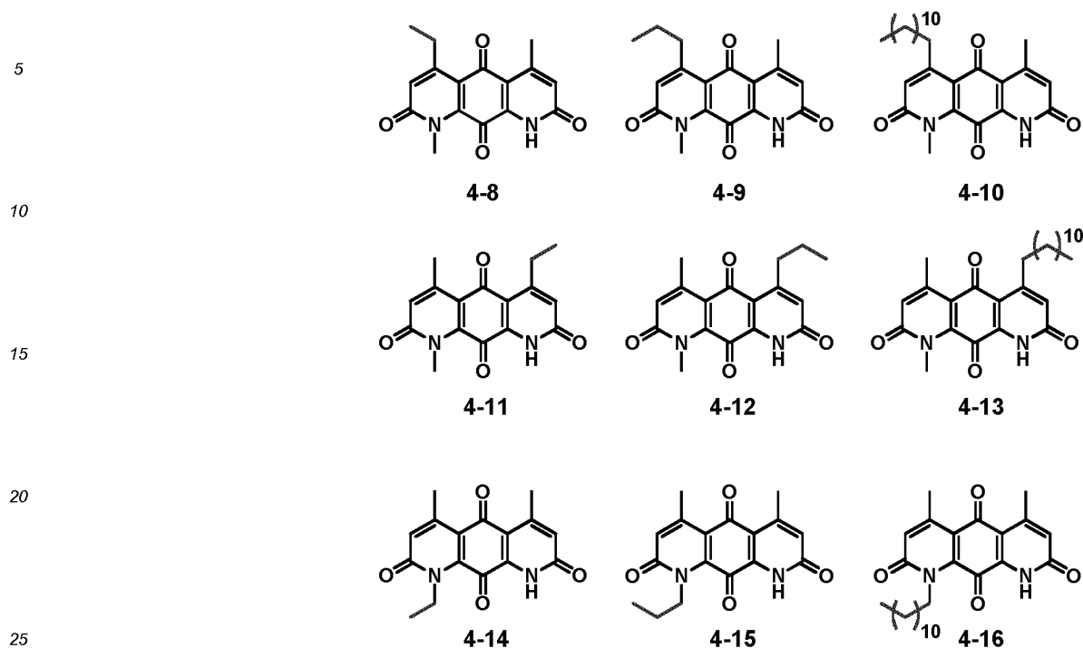
Scheme 4.1. Nine DNQ derivatives.
