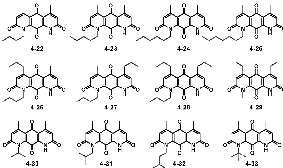
Scheme 4.3. New DNQ derivatives.
