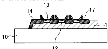
B-B' CROSS SECTION VIEW
