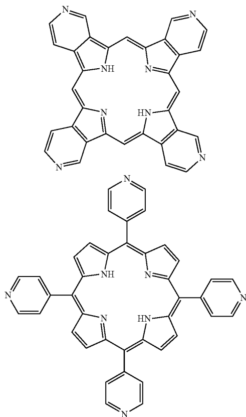
4,4',4'',4'''-tetraaza-29H,31H-phthalocyanine 5,10,15,20-Tetra(4-pyridyl)-21H,23H-porphine
