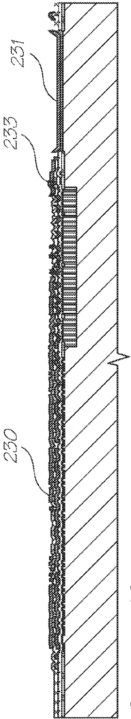
Deposit metal 2
