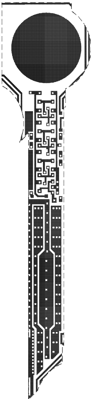
Metal 1 mask
