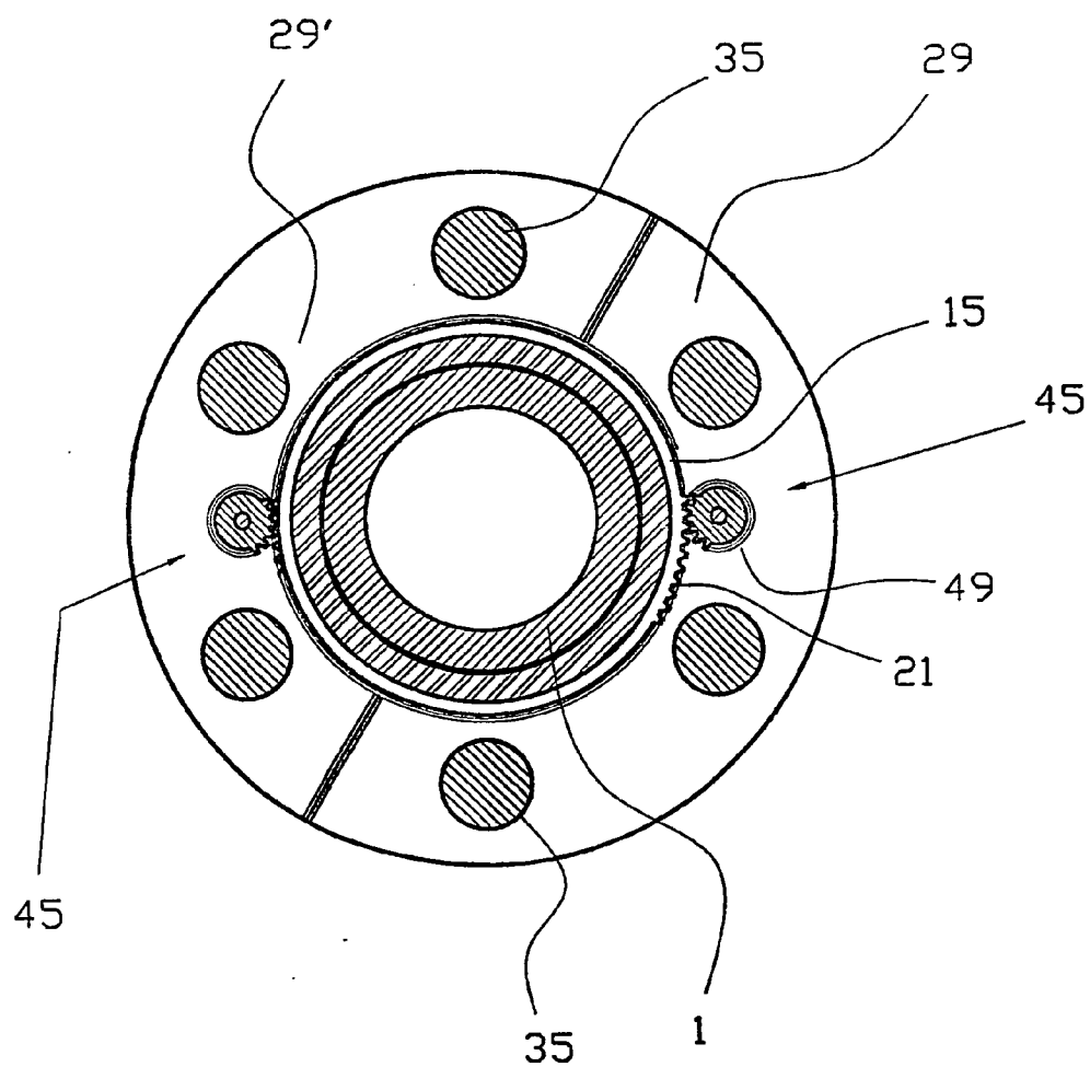
Cross section 2-2
