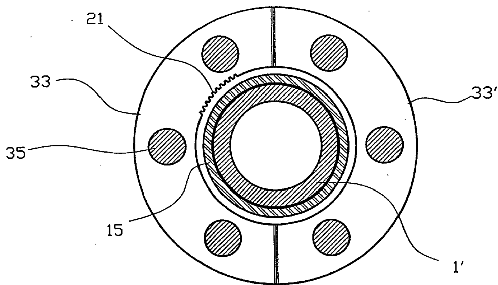
Cross section 1-1
