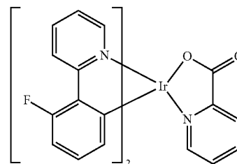
[F 2 Irpic]
