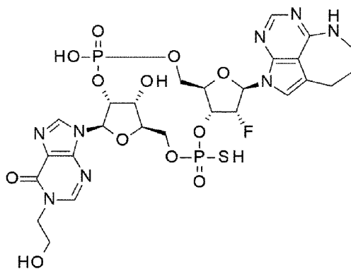
53 53a (Diastereomer 1)
