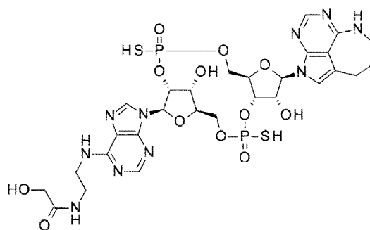
15 15a (Diastereomer 1)
