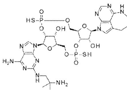
10 10a (Diastereomer 1)
