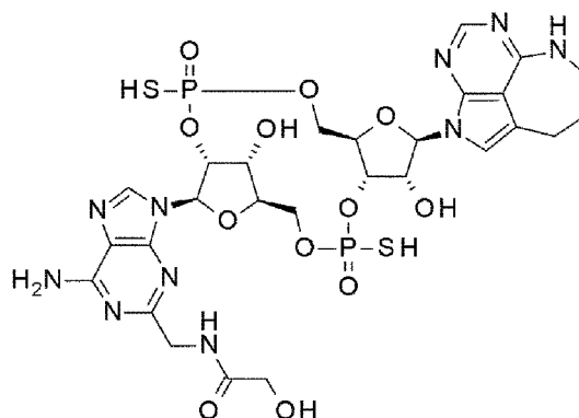
29 29a (Diastereomer 1)
