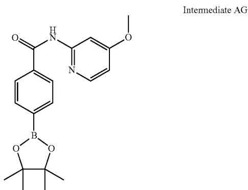
N-(4-methoxypyridin-2-yl)-4-(4,4,5,5-tetramethyl-1,3,2-dioxaborolan-2-yl)benzamide
