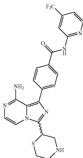
4-(8-amino-3-(thiomorpholin-2-yl)imidazo[1,5-a] pyrazin-1-yl)-N-(4-(trifluoromethyl)-pyridin-2-yl) benzamide
