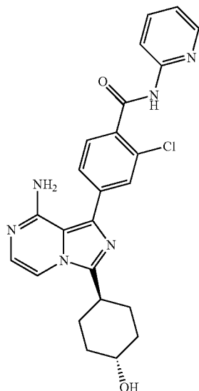
4-(8-amino-3-((trans)-4-hydroxycyclohexyl)imidazo [1,5-a]pyrazin-1-yl)-2-chloro-N-(pyridin-2-yl)benz- amide
