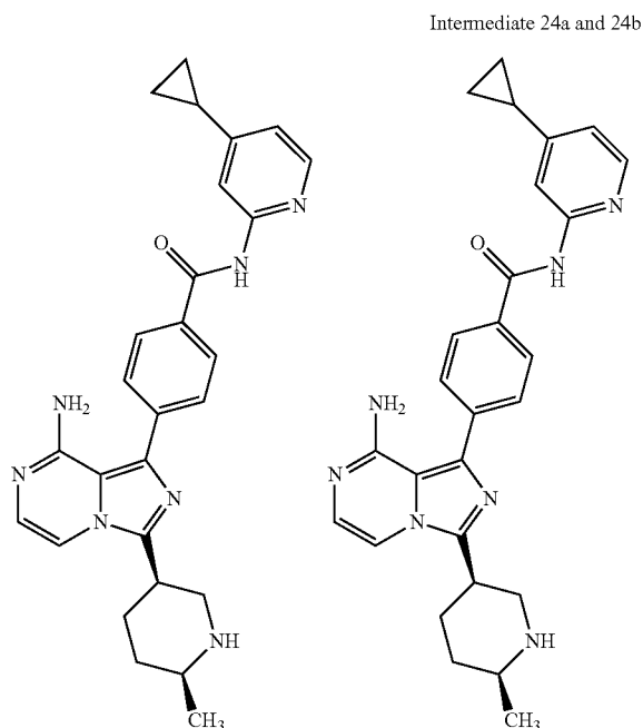
4-(8-amino-3-((cis)-6-methylpiperidin-3-yl)imidazo[1,5-a]pyrazin-1-yl)-N-(4-cyclopropylpyridin-2-yl)benzamide and 4-(8-amino-3-((trans)-6-methylpiperidin-3-yl)imidazo[1,5-a]pyrazin-1-yl)-N-(4-cyclopropylpyridin-2-yl)benzamide
