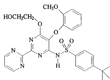
(Bosentan)
