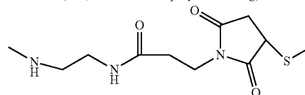
(MP, maleimidopropanoyl containing)
