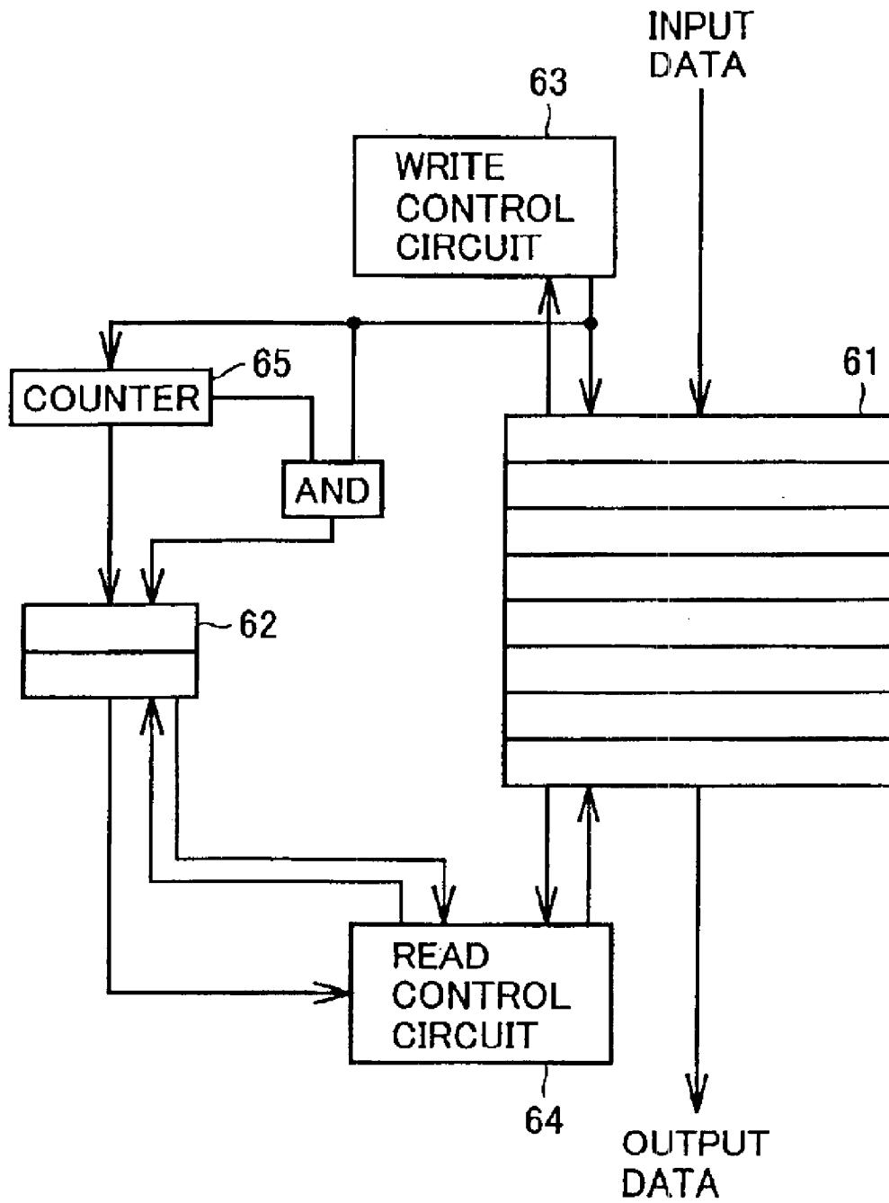
FIG.20 PRIOR ART
