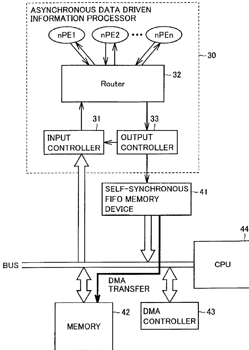
FIG.18 PRIOR ART
