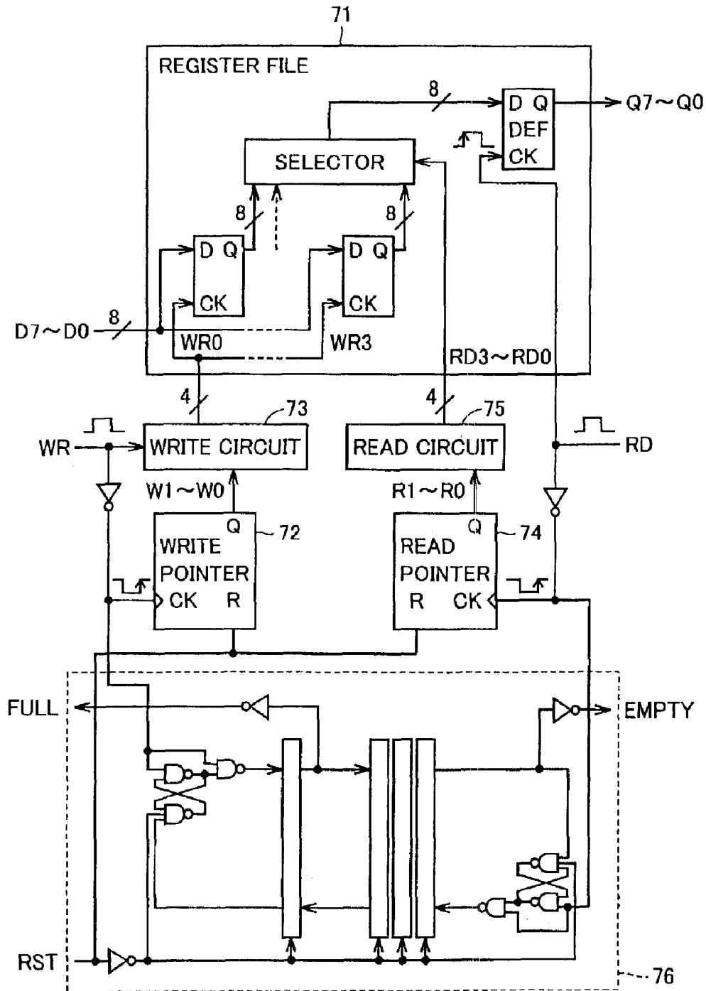
FIG.21 PRIOR ART
