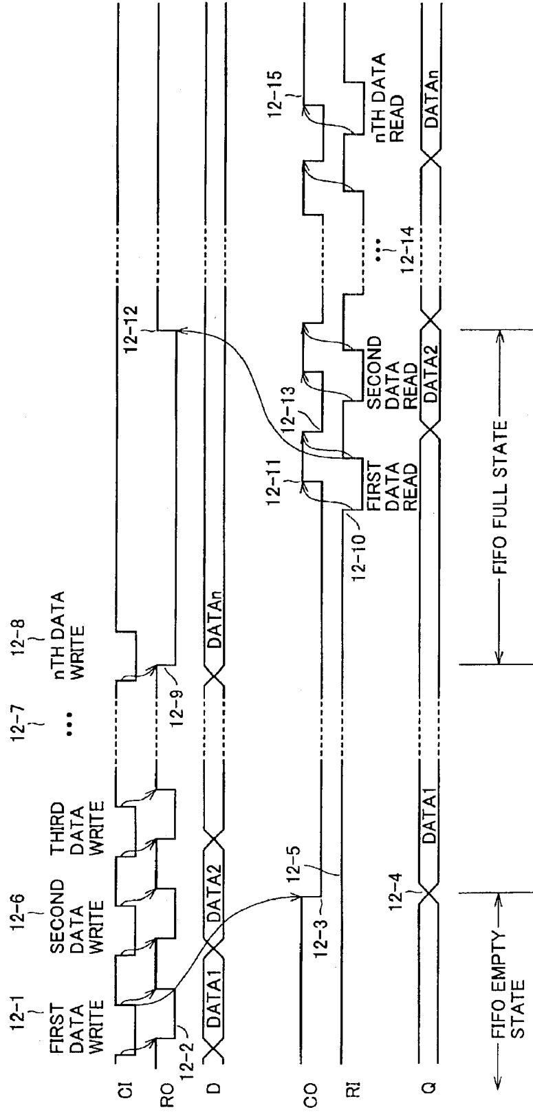
FIG.17 PRIOR ART
