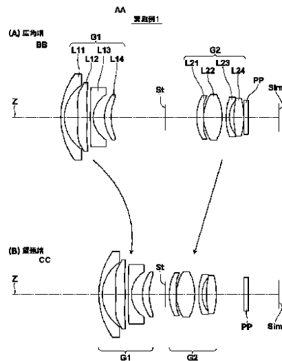
AA Embodiment 1 BB (A) Wide angle end CC (B) Telescopic end
