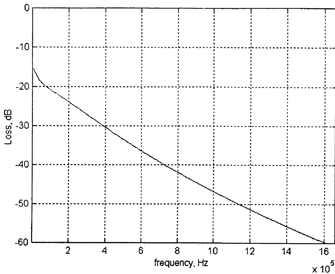
Transfer Function 6000 feet 26 AWG telephone cable
