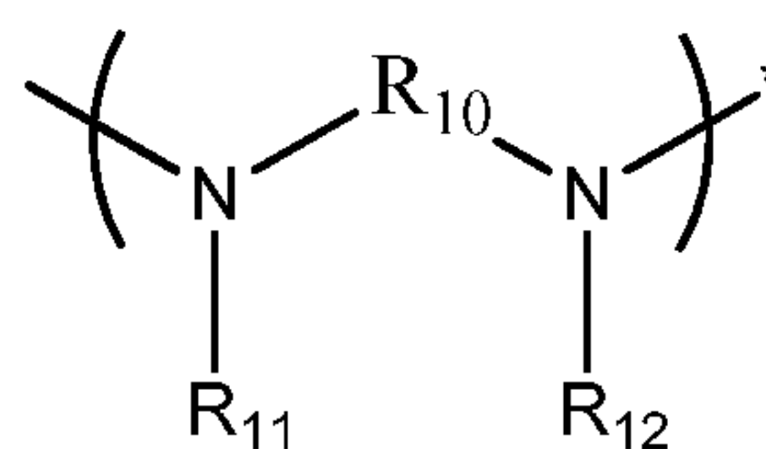
Formula 30
