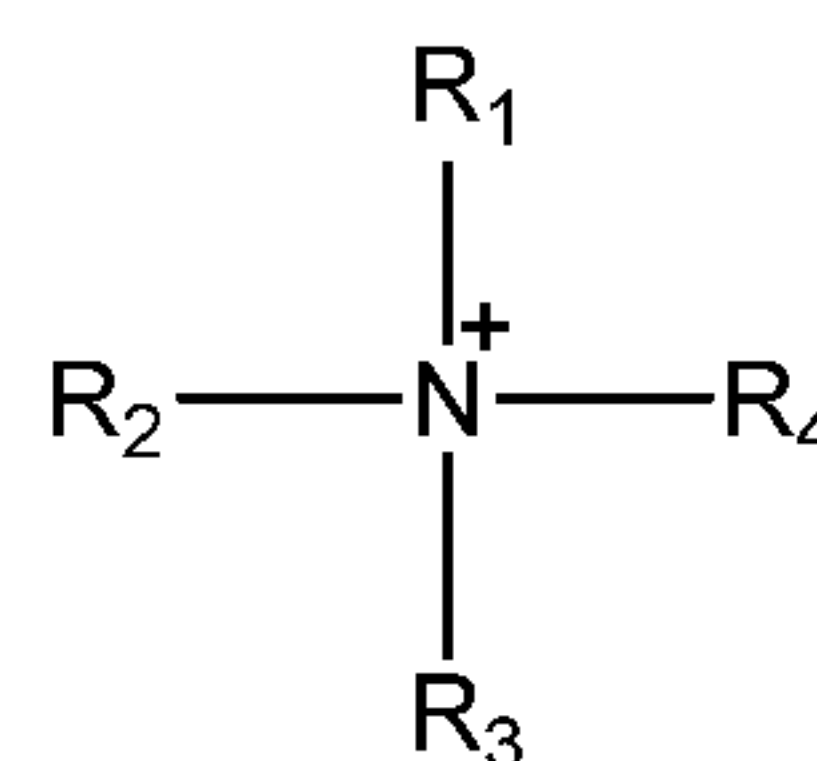
Formula 2
