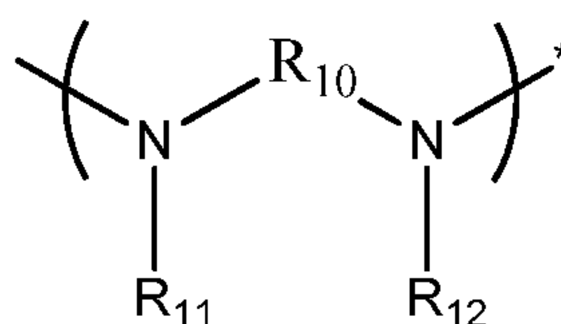
Formula 30
