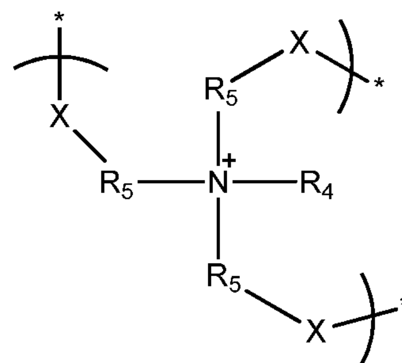
Formula 20
