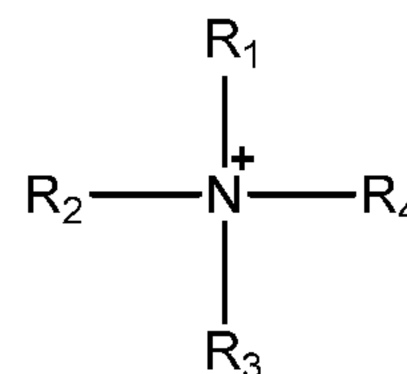
Formula 2
