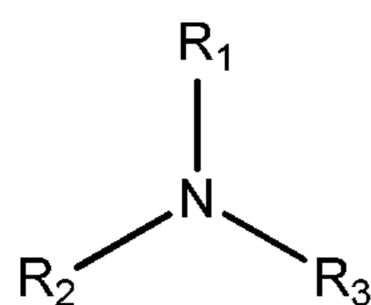
Formula 1
