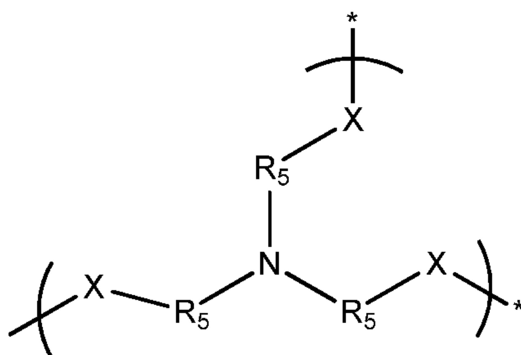
Formula 10
