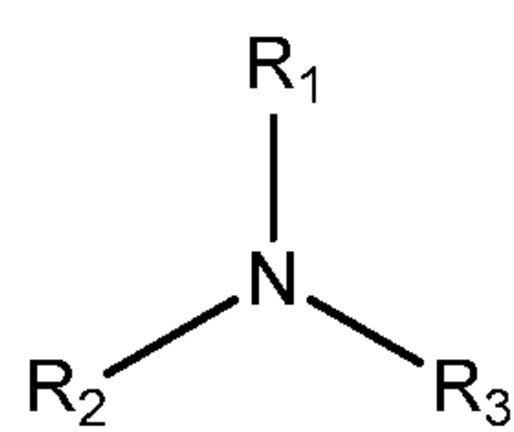
Formula 1
