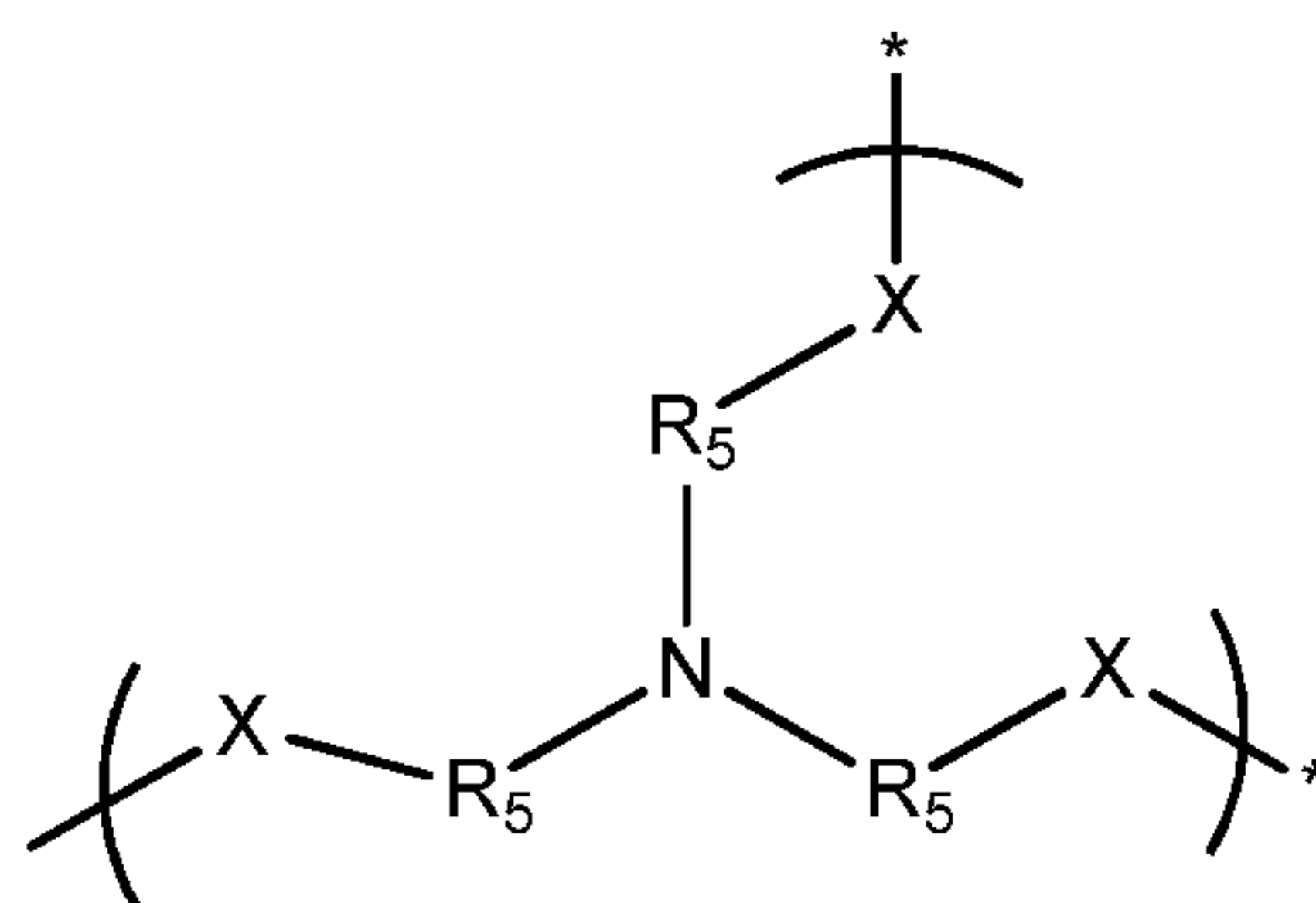
Formula 10
