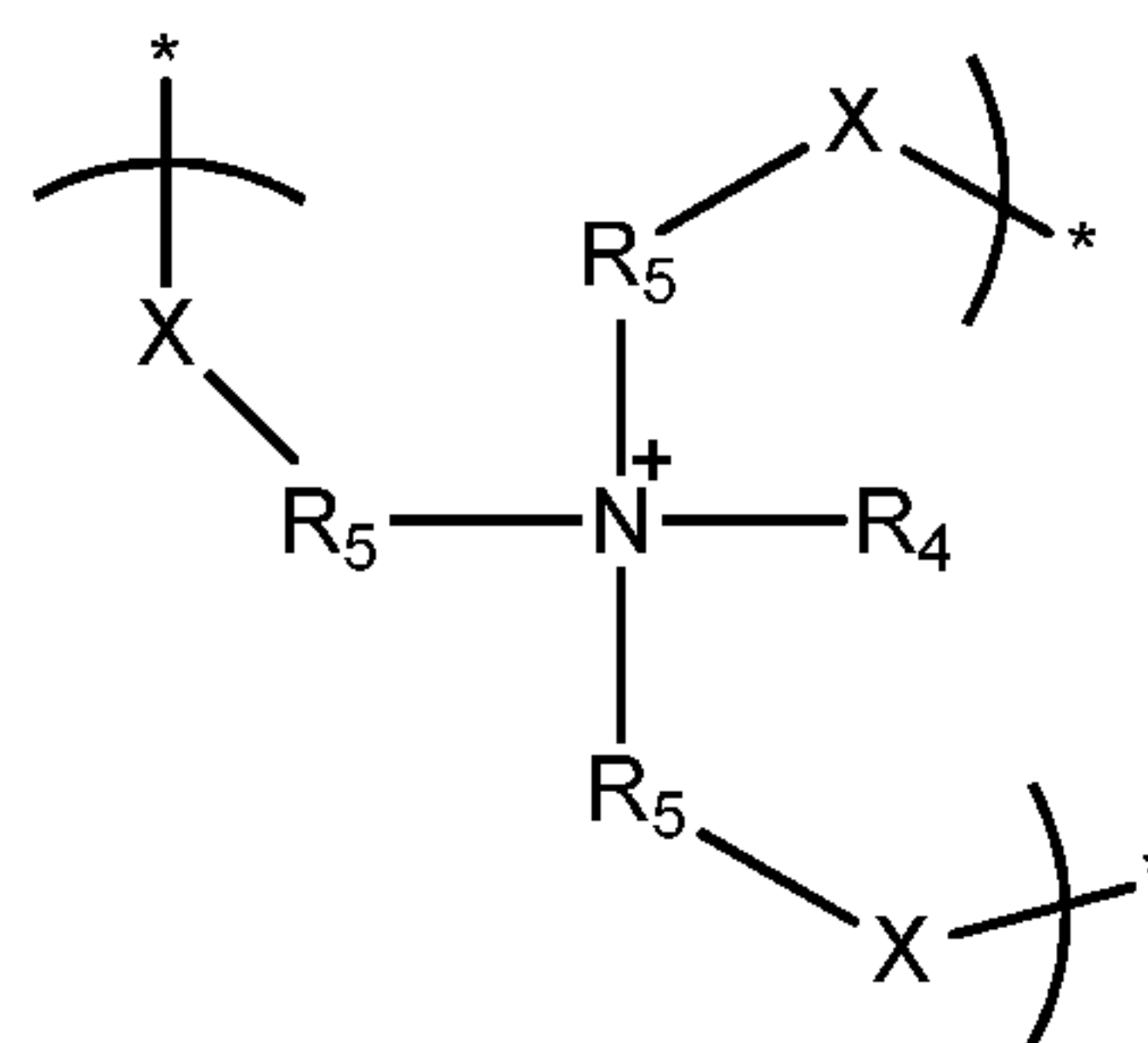
Formula 20
