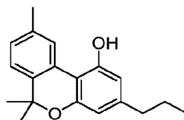
cannabivarin [CBN-C 3 ]
