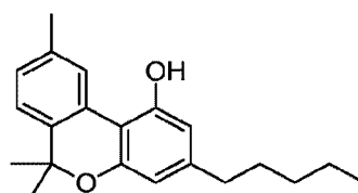
cannabinol [CBN]
