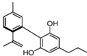
cannabinodivarin [CBND-C 3 ]
