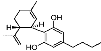
cannabidiol-C 4 [CBD-C 4 ]
