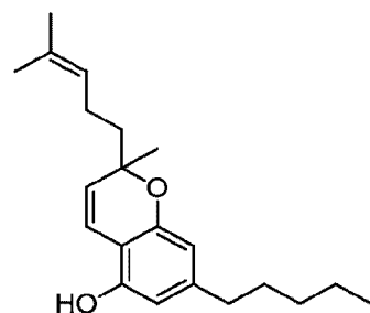
(±)-cannabichromene [CBC]
