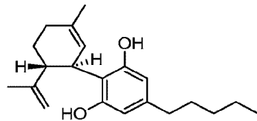
(-)-cannabidiol [CBD]
