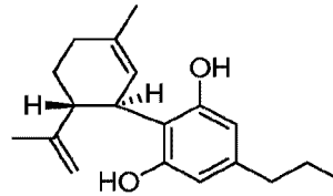
(-)-cannabidivarin [CBDV]
