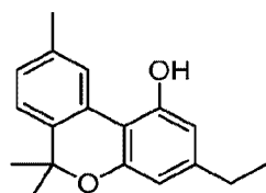
cannabinol-C 2 [CBN-C 2 ]
