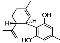
cannabiorcol [CBD-D 1 ]
