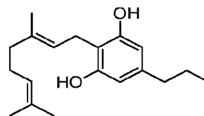
cannabigerovarin [CBGV]
