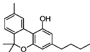
cannabinol-C 4 [CBN-C 4 ]
