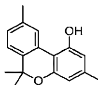
cannabiorcol [CBN-C 1 ]
