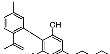
cannabinodiol [CBND]
