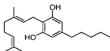
cannabigerol [CBG]
