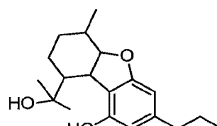
cannabiglendol-C 3 [OH-iso-HHCV-C 3 ]
