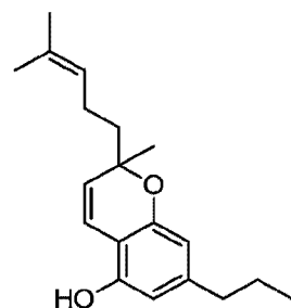
(±)-cannabichromevarin [CBCV]
