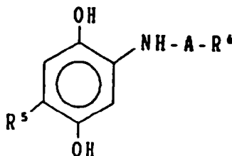
Formula (RD-1)
