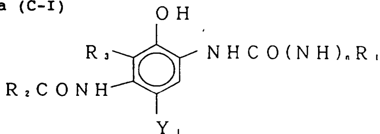
Formula (C-I)
