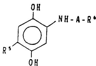
Formel (RD-1)
