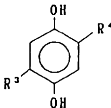
Formula (HQ-2)
