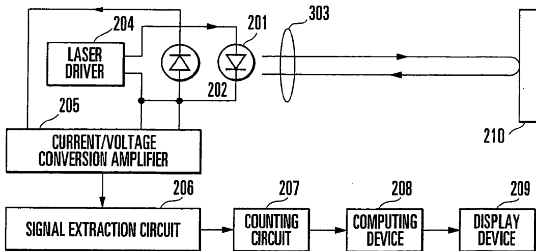
FIG. 15 PRIOR ART
