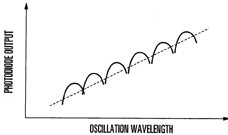
FIG. 14 PRIOR ART
