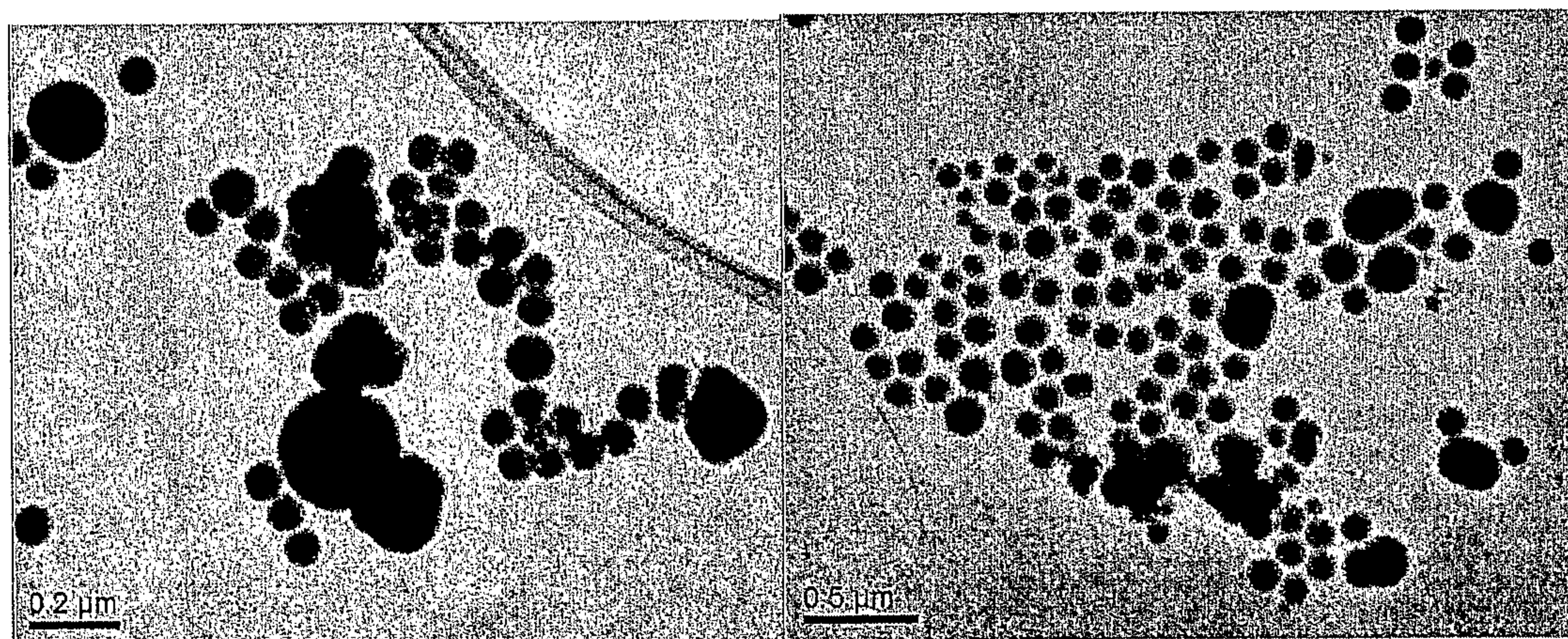
e: core+4-layer (bar=200 nm)
