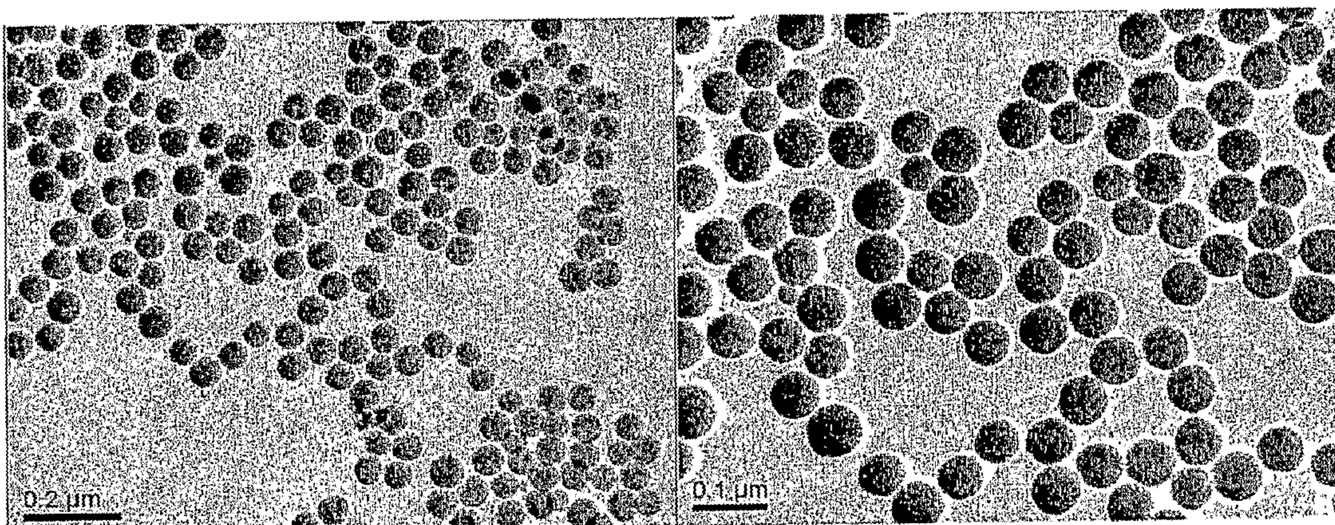
b: core+1-layer (bar=200 nm)
