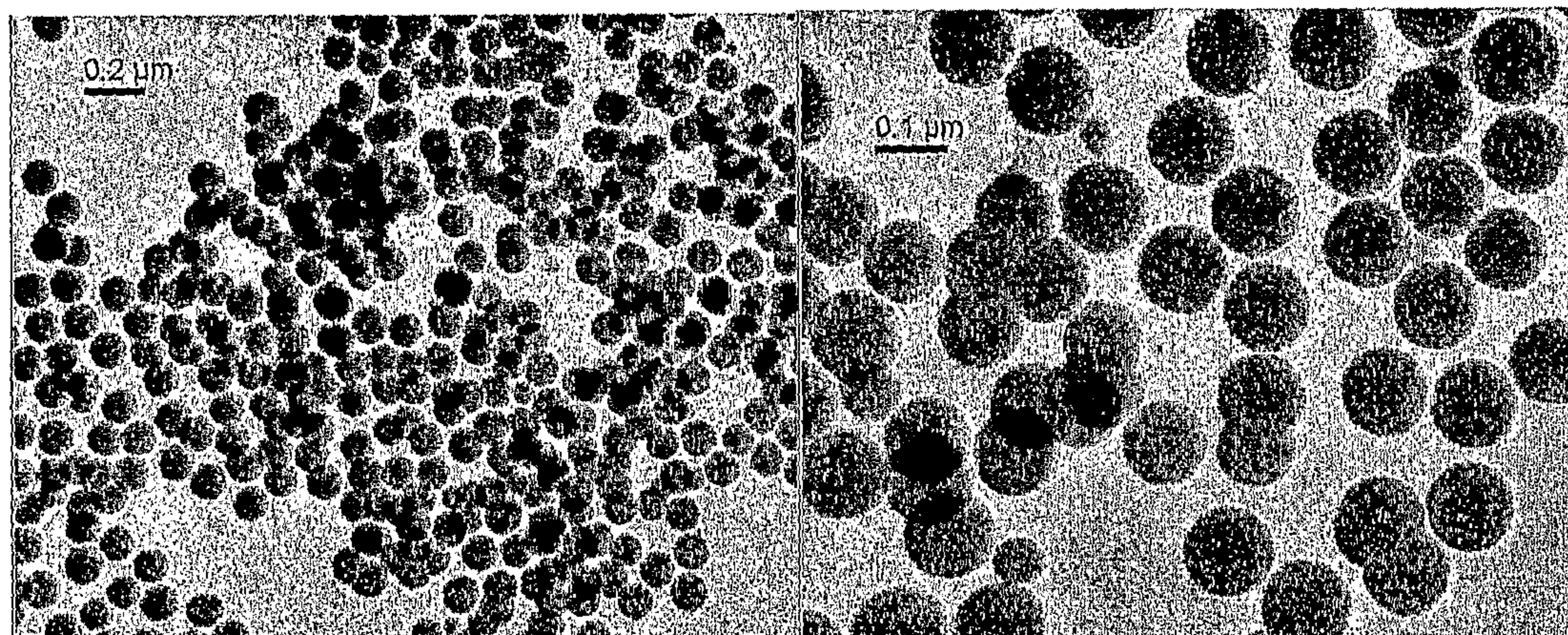
d: core+3-layers (bar=200 nm)
