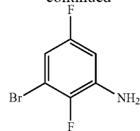
3-bromo-2,5-difluoroaniline
