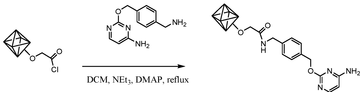
Scheme 7.
