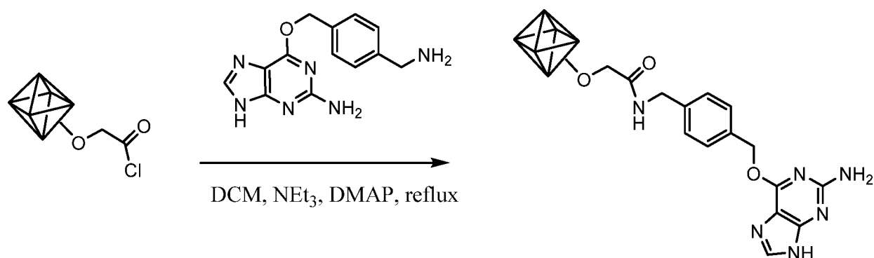
Scheme 6.
