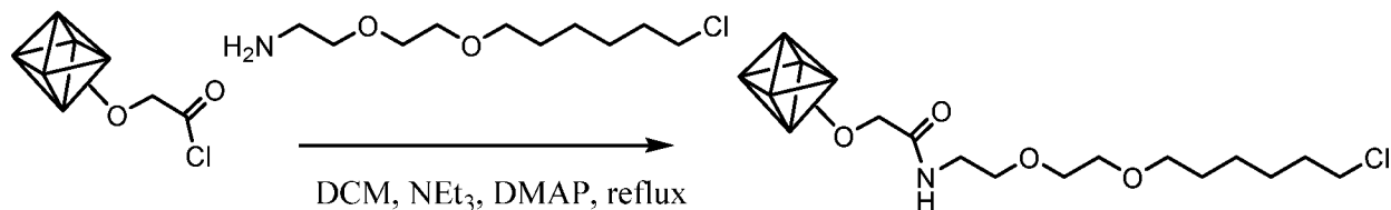
Scheme 5.
