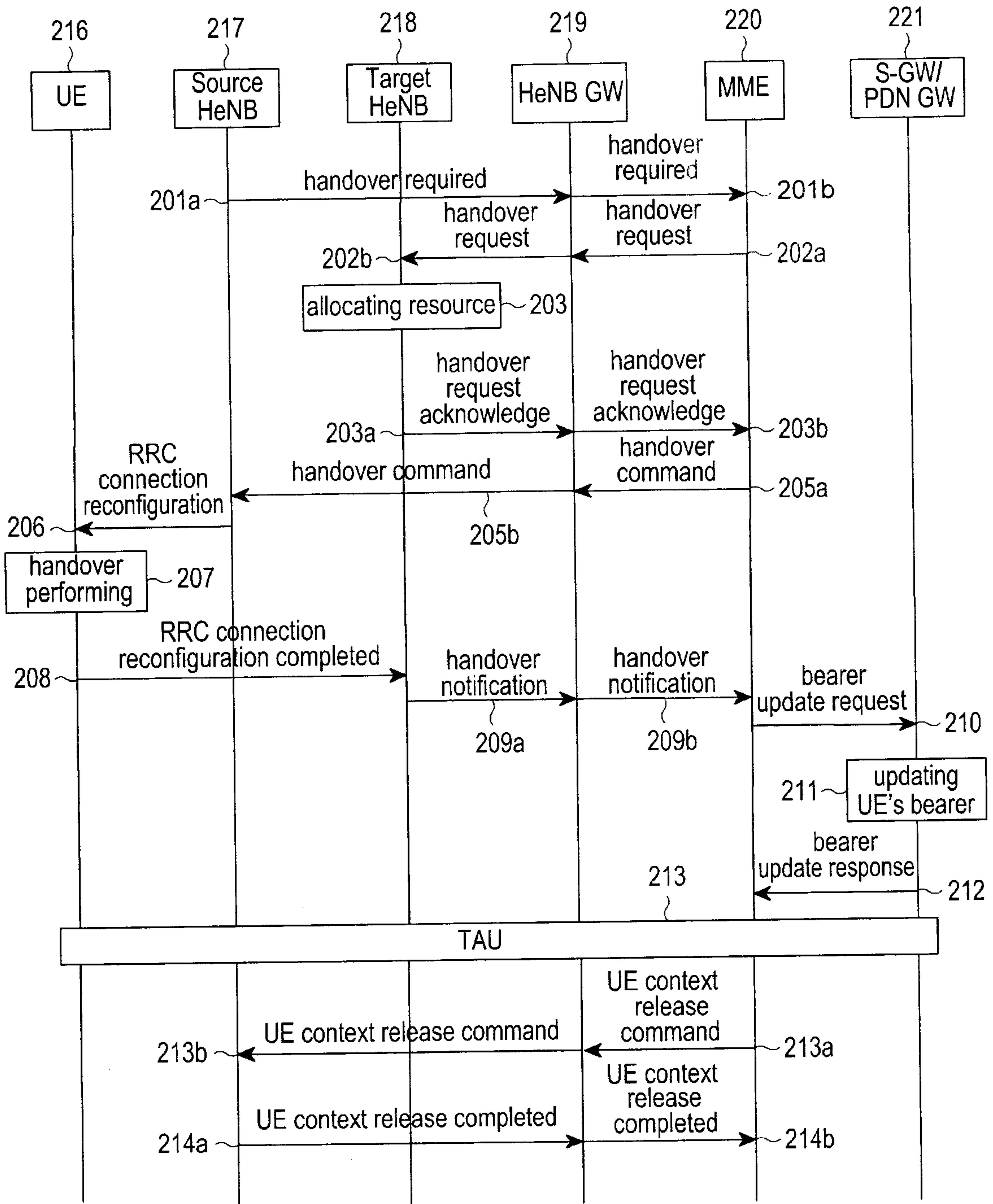
FIG.2 (RELATED ART)
