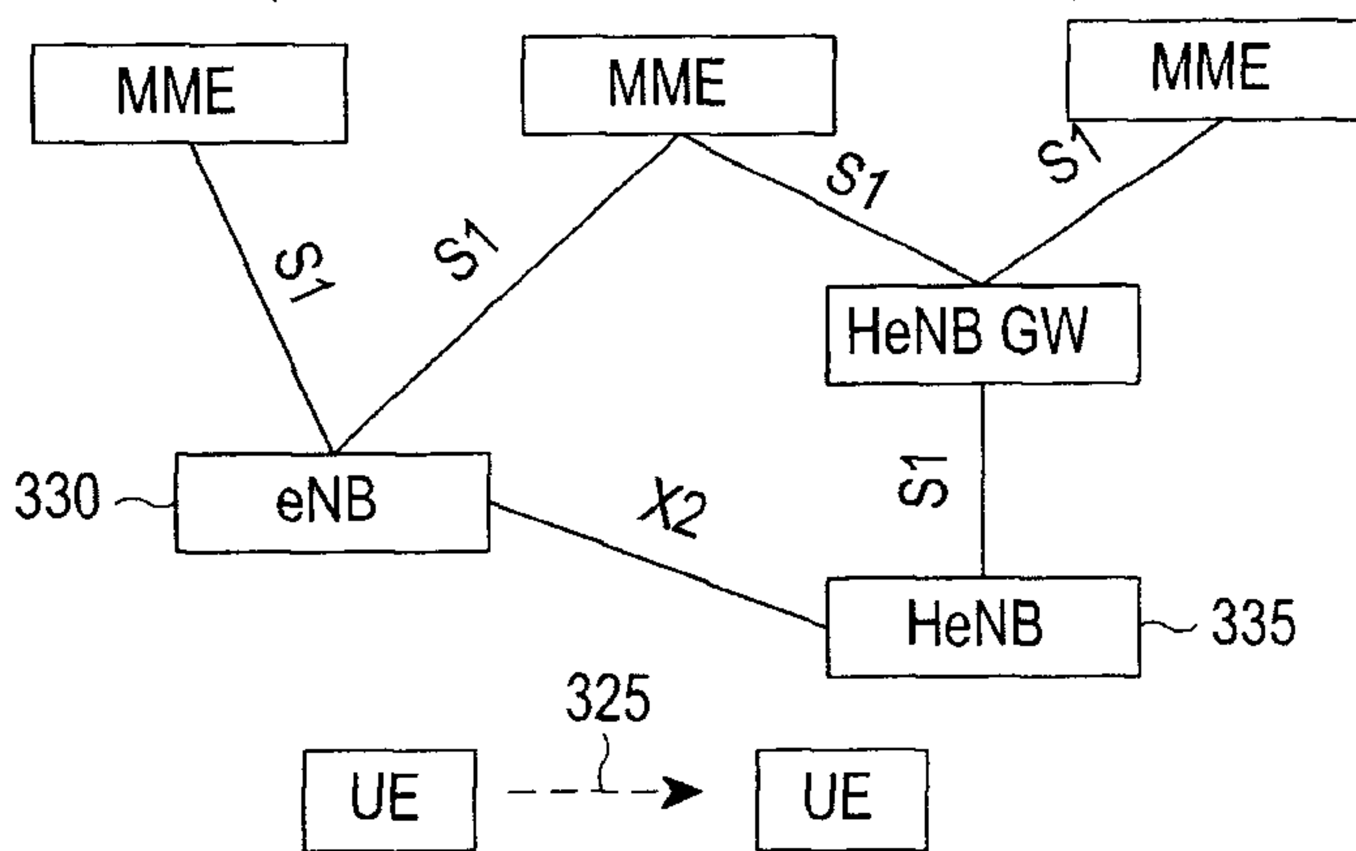
FIG.3C (RELATED ART)
