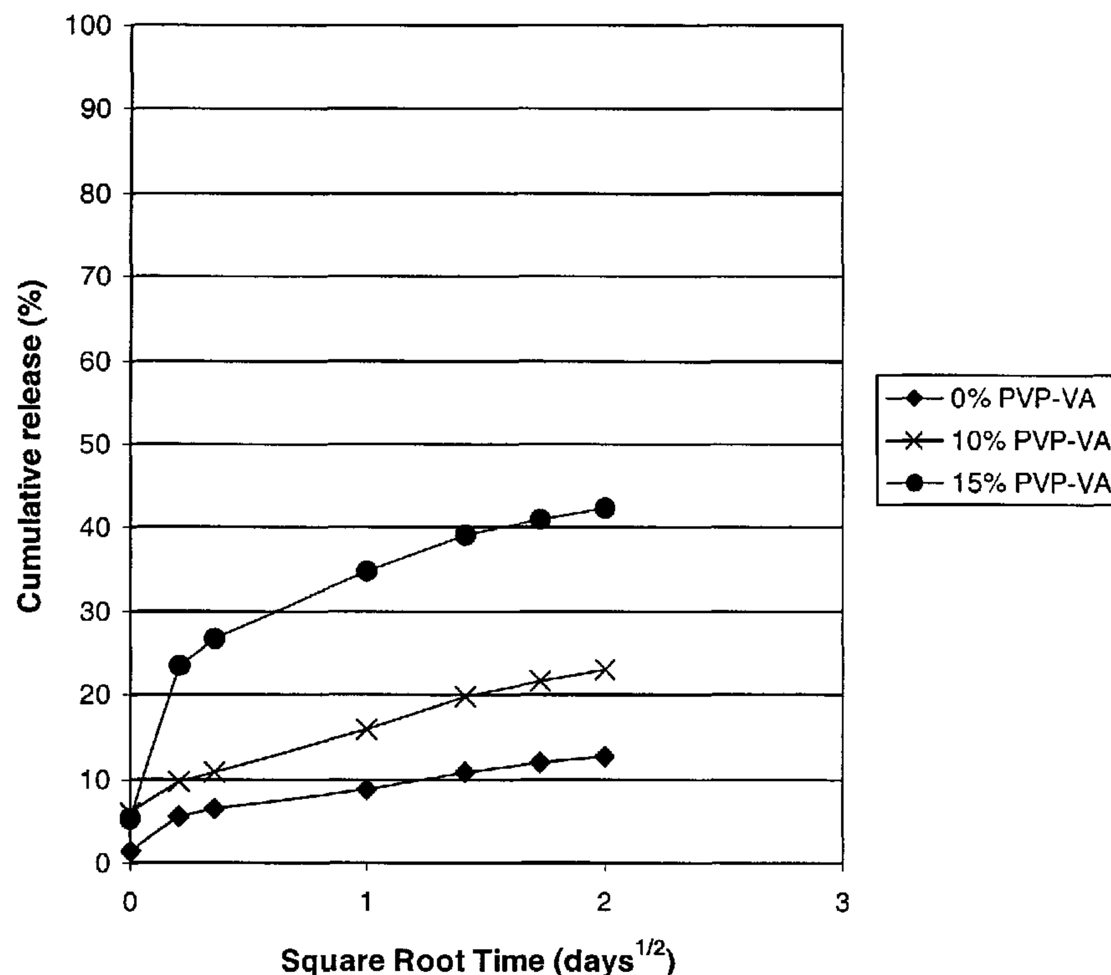
Resten NG delivery from Tecophilic / PVP-VA matrix
