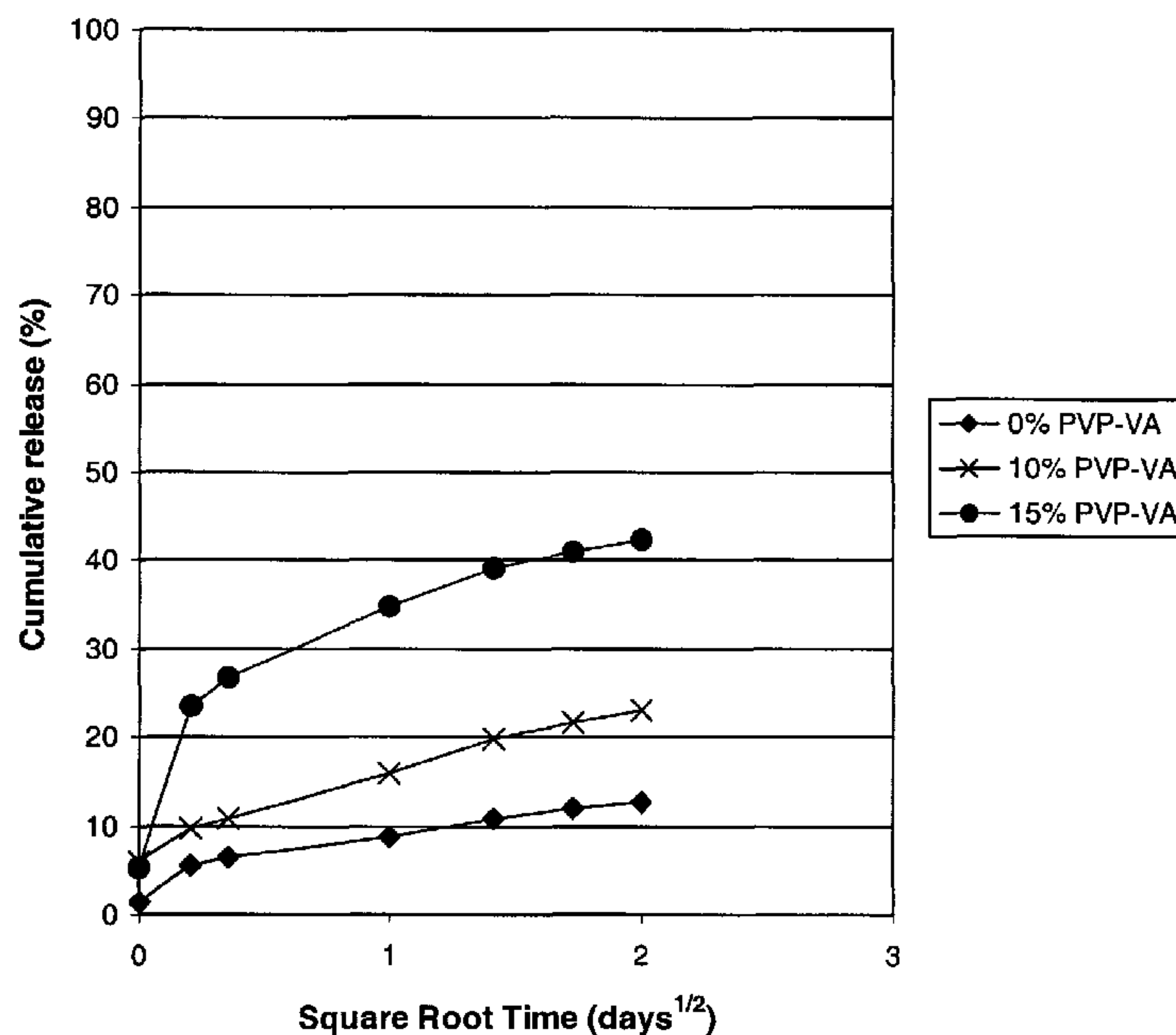
Resten NG delivery from Tecophilic / PVP-VA matrix
