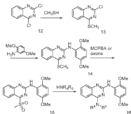
Scheme 7: Synthesis of exemplary compounds of Formula (VIII)
