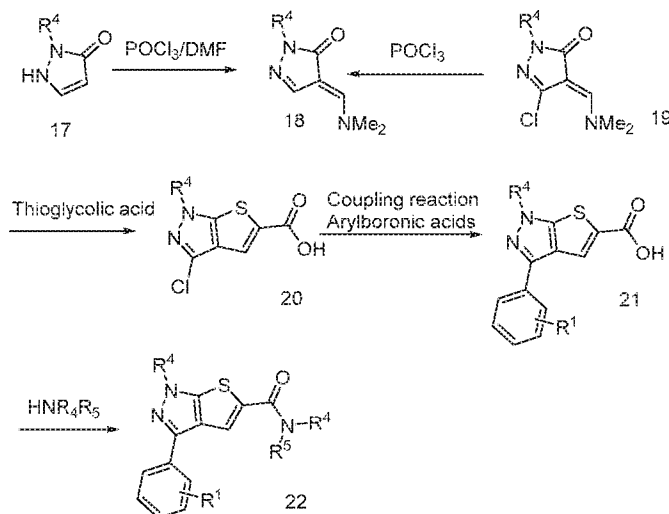
Scheme 8: Synthesis of exemplary compounds of Formula (IX)
