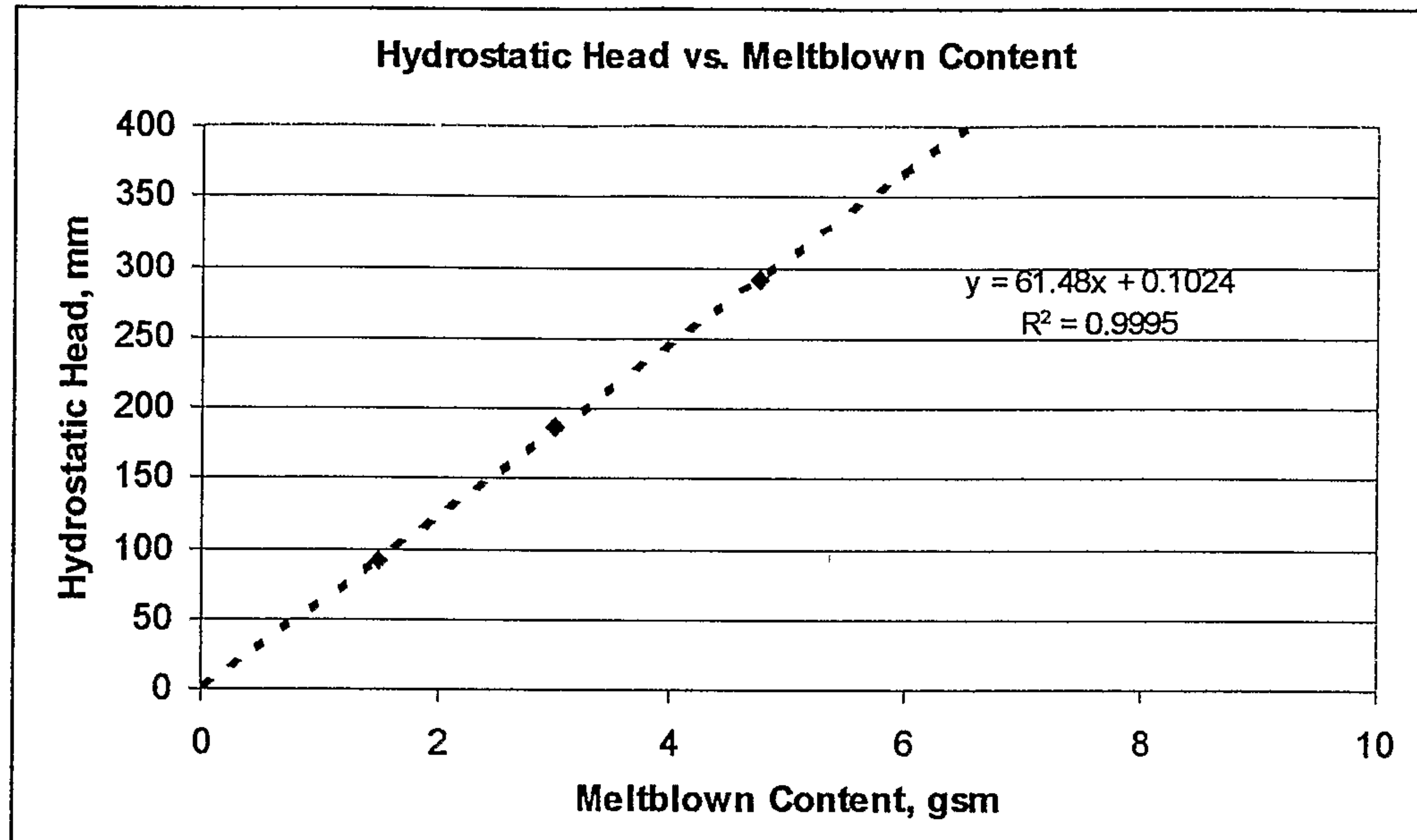
Figure 1. Graph of Hydrostatic Head versus Meltblown Content of Barrier-Coated SMS Carriers
