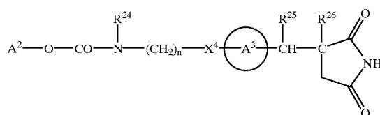
Formula VII
