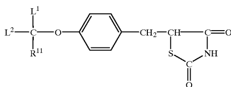
Heterocyclic Group
