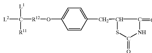
Formula II(a)
