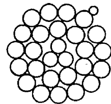
FIG.4c PRIOR ART
