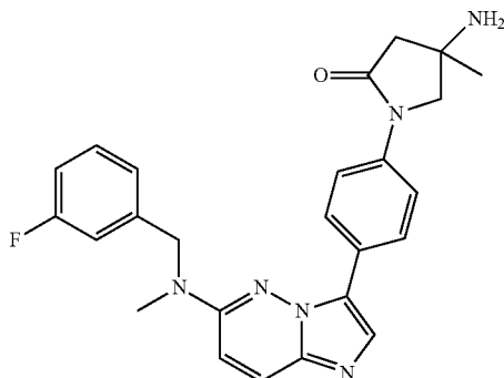
4-Amino-1-[4-[6-[(3-fluorophenyl)methyl-methyl-amino]imidazo[1,2-b]pyridazin-3-yl]phenyl]-4-methylpyrrolidin-2-one
