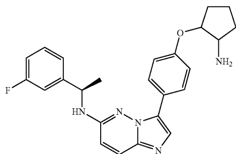
3-[4-(cis-2-Aminocyclopentoxy)phenyl]-N- [(1R)-1-(3-fluorophenyl)ethyl]imidazo[1,2- b]pyridazine-6-amine
