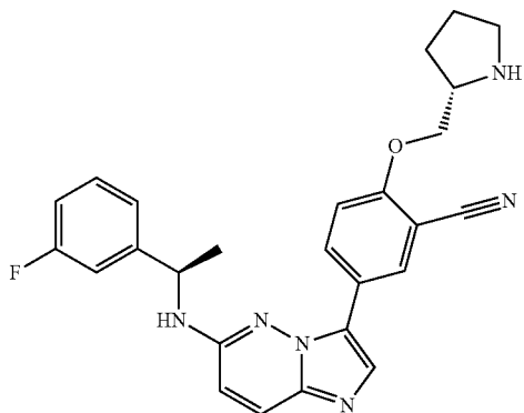
5-[6-[[[(1R)-1-(3- Fluorophenyl)ethyl]amino]imidazo [1,2-b]pyridazin-3-yl]-2-[[[(2S)- pyrrolidin-2- yl]methoxy]benzonitrile
