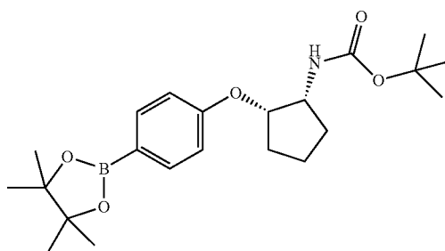
tert-Butyl N-[(1R,2S)-2-[4-(4,4,5,5-tetramethyl-1,3,2-dioxaborolan-2-yl)phenoxy]cyclopentyl]carbamate
