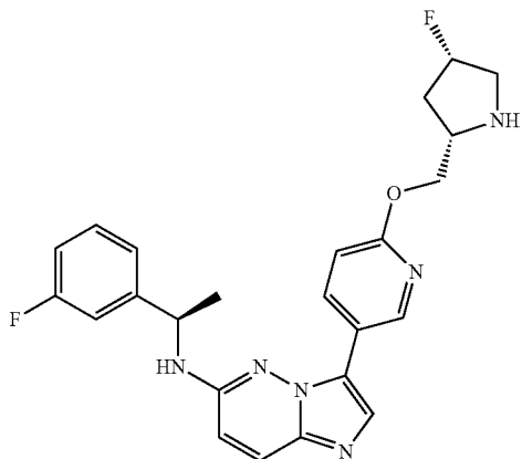
N-[(1R)-1-(3-Fluorophenyl)ethyl]- 3-[6-[[[(2S,4S)-4-fluoropyrrolidin- 2-yl]methoxy]-3- pyridyl]imidazo[1,2-b]pyridazin-6- amine
