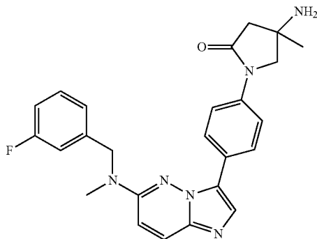
4-Amino-1-[4-[6-[(3-fluorophenyl)methyl-methyl-amino]imidazo[1,2-b]pyridazin-3-yl]phenyl]-4-methylpyrrolidin-2-one
