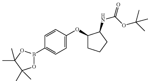
tert-Butyl N-[(1S,2R)-2-[4-(4,4,5,5-tetramethyl-1,3,2-dioxaborolan-2-yl)phenoxy]cyclopentyl]carbamate
