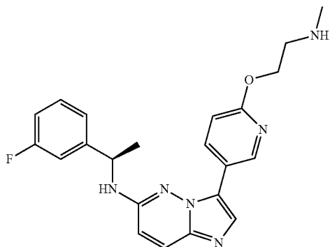
N-[(1R)-1-(3-Fluorophenyl)ethyl]- 3-[6-[2-(methylamino)ethoxy]-3- pyridyl]imidazo[1,2-b]pyridazin-6- amine
