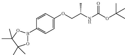
tert-Butyl N-[(1S)-1-methyl-2-[4-(4,4,5,5-tetramethyl-1,3,2-dioxaborolan-2-yl)phenoxy]ethyl]carbamate
