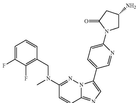
(4S)-4-Amino-1-[5-[6-[(2,3-difluorophenyl)methyl-methylamino]imidazo[1,2-b]pyridazin-3-yl]-2-pyridyl]pyrrolidin-2-one
