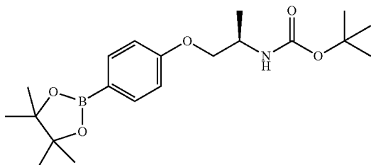
tert-Butyl N-[(1R)-1-methyl-2-[4-(4,4,5,5-tetramethyl-1,3,2-dioxaborolan-2-yl)phenoxy]ethyl]carbamate
