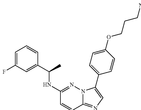
3-[4-(3-Aminopropoxy)phenyl]-N-[(1R)-1-(3-fluorophenyl)ethyl]imidazo[1,2-b]pyridazin-6-amine
