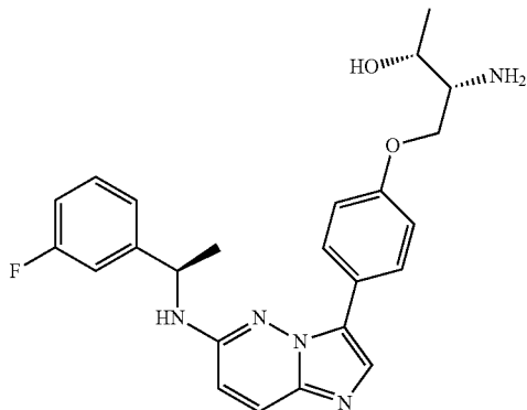
(2R,3R)-3-Amino-4-[4-[6-[(1R)-1-(3-fluorophenyl)ethyl]amino]imidazo[1,2-b]pyridazin-3-yl]phenoxy]butan-2-ol
