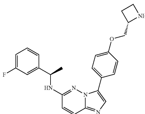
3-[4-[(2S)-Azetidin-2-yl]methoxy]phenyl]-N-[(1R)-1-(3-fluorophenyl)ethyl]imidazo[1,2-b]pyridazin-6-amine
