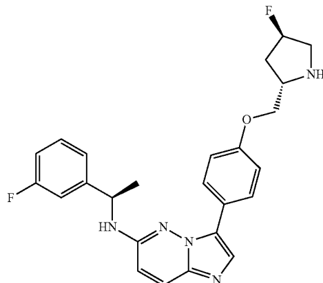
N-[(1R)-1-(3-Fluorophenyl)ethyl]- 3-[4-[(2S,4S)-4-fluoropyrrolidin- 2-yl]methoxy]phenyl]imidazo[1,2- b]pyridazine-6-amine
