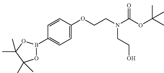
tert-Butyl N-(2-hydroxyethyl)-N-[2-[4-(4,4,5,5-tetramethyl-1,3,2-dioxaborolan-2-yl)phenoxy]ethyl]carbamate
