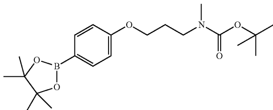
tert-Butyl N-methyl-N-[3-[4-(4,4,5,5-tetramethyl-1,3,2-dioxaborolan-2-yl)phenoxy]propyl]carbamate
