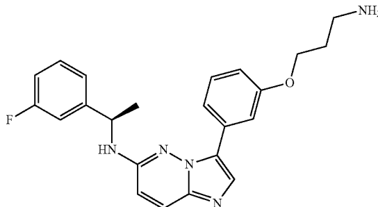
3-[3-(3-Aminopropoxy)phenyl]-N-[(1R)-1-(3-fluorophenyl)ethyl]imidazo[1,2-b]pyridazin-6-amine
