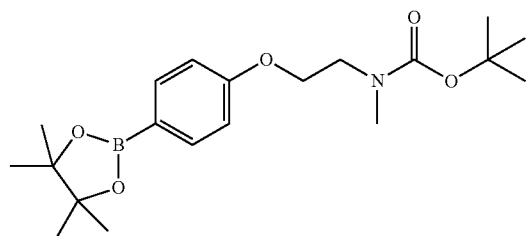
tert-Butyl N-methyl-N-[2-[4-(4,4,5,5-tetramethyl-1,3,2-dioxaborolan-2-yl)phenoxy]ethyl]carbamate
